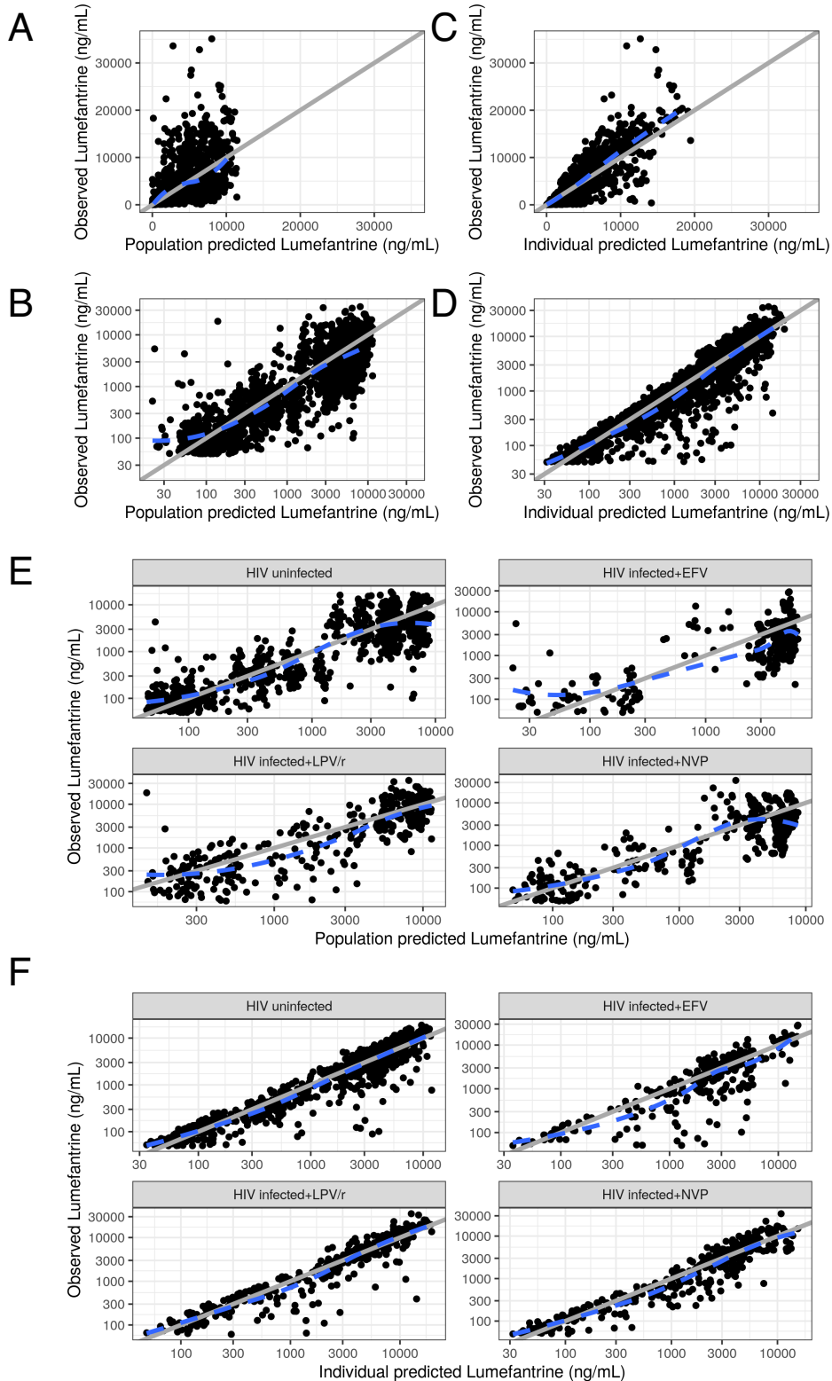
Figure S3. Model observations versus predictions. Observed values for the entire cohort, indicated by solid black circles, for population (A, B, top left) and individual (C, D, top right) predictions on a linear- (A, C) and log-scale (B, D). Observed values stratified by HIV status and ART regimen for population (E, middle) and individual (F, bottom) predictions on a log-scale. The line of identity (solid grey) is included as a reference ( x=y ). The dashed blue line represents a LOESS smooth through the data.
