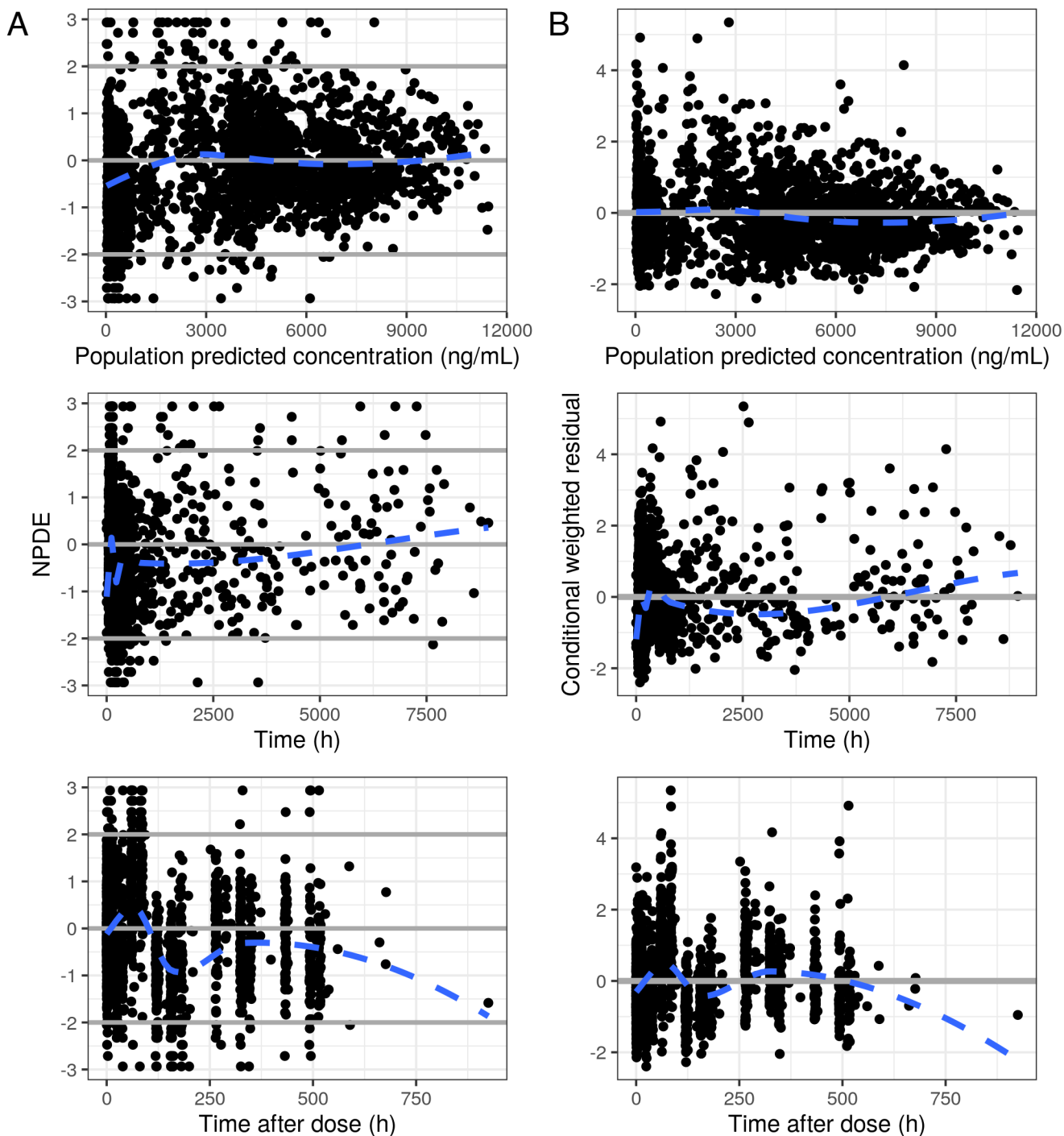
Figure S4: Normalized prediction distribution errors (NPDE) and conditional weighted residuals (CWRES) versus population predictions, time, and time after dose. Solid black circles represent the individual NPDE values (A, left plots) and CWRES values (B, right plots) associated with each observation record. The solid horizontal grey lines (residuals = -2, 0, 2 for NPDE and residuals = 0 for CWRES) were included for reference. The dashed blue line represents a LOESS smooth through the data.
