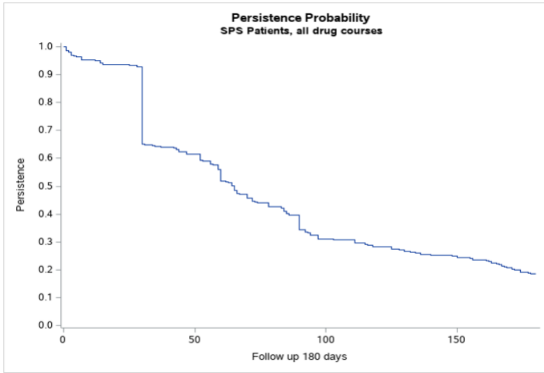
Supplemental Figure 3. Patiromer persistence probability for all courses in the full study population
