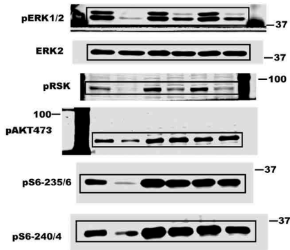
2B: MOLM13
