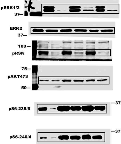
2C: MOLM14
