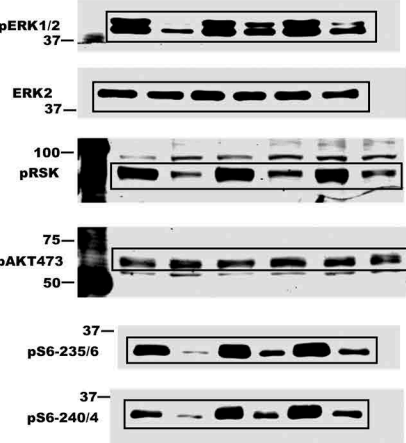
2C: MV4-11
