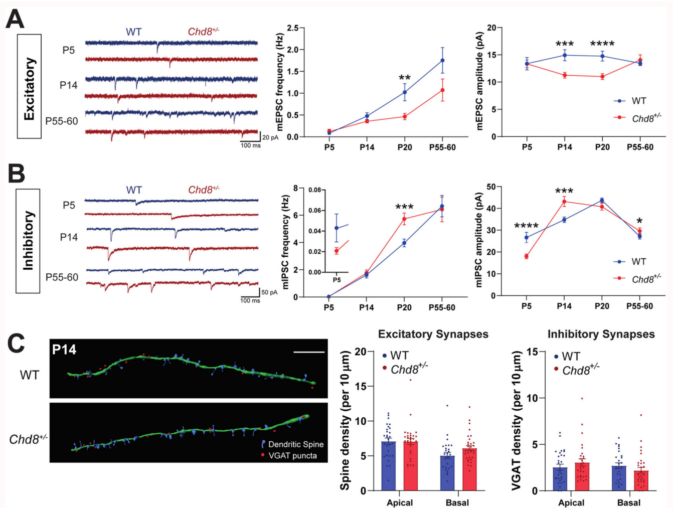
Fig. 2. Developmental stage-specific synaptic effects of Chd8 heterozygosity.
