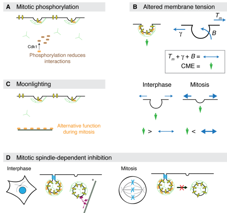
Figure 2. Four mechanisms proposed to account for CME shutdown during mitosis
