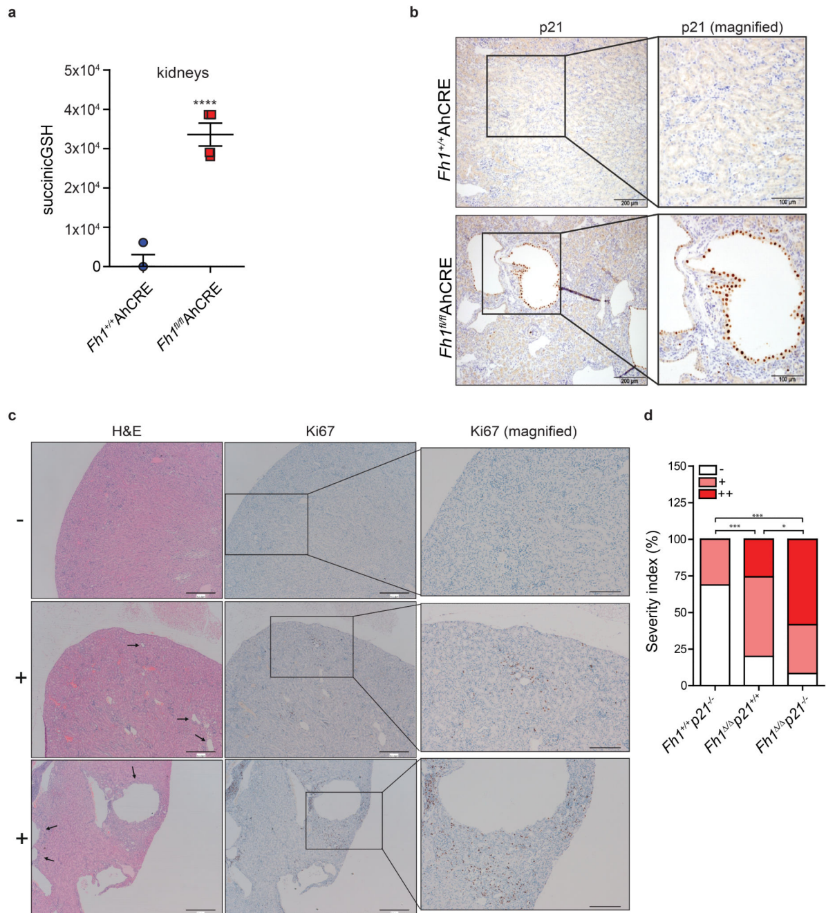
Figure 7. GSH succination is associated with fumarate-induced senescence in renal cysts (a) SuccinicGSH was measured in kidney extracts of the indicated animals by LC-MS. Four animals for each genotype were used for this experiment. (b) Representative images of p21 immunostaining performed on dissected kidneys of the indicated mice. (c) Representative H&E staining and Ki67 immunostaining images of the different histological grading of kidney hyperplasia observed in 12-18 month-old mice. Representative images from normal kidneys, scored as (-), were taken from Fh1^{+/+} p21^{-/-} animals; kidneys with limited number of cysts (arrows) and areas of hyperplasia with low overall Ki67, staining scored as (+),
