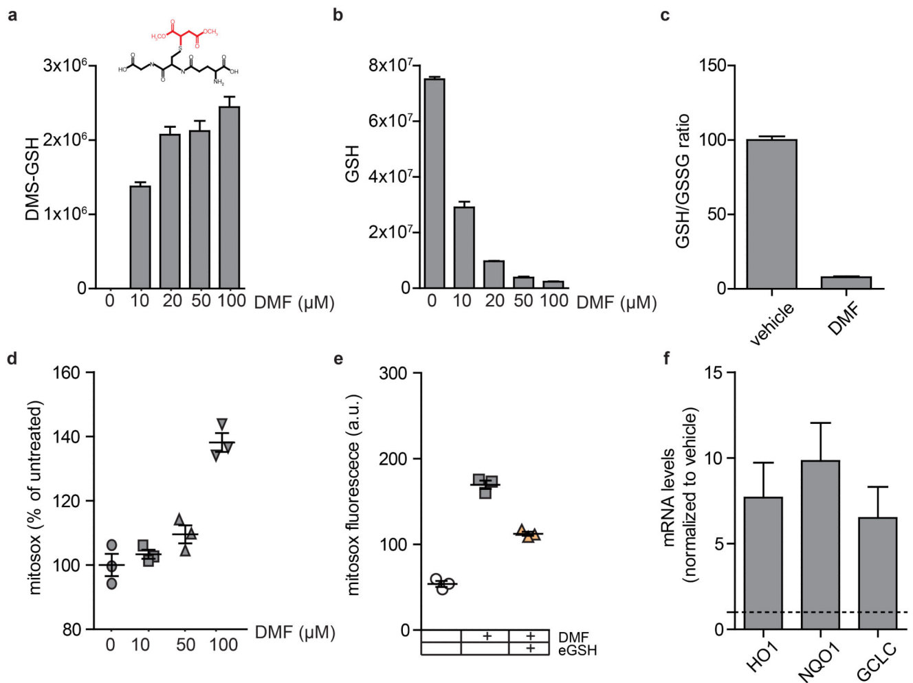
Figure 4. Dimethyl-fumarate induces GSH succination and increases oxidative stress (a-c) Cell-permeable dimethyl-fumarate (DMF) binds to (a) and depletes (b) the intracellular pool of GSH, leading to a decrease in GSH/GSSG ratio (c). The structure of the adduct between GSH and DMF, DMS-GSH, is indicated in panel (a). (d-f) DMF induces oxidative stress (d-e) and the activation of an antioxidant response, measured by the expression of antioxidant genes (f). The redox stress caused by DMF is attenuated by incubating cells with a cell permeable derivative of GSH, eGSH (e). HO1 = heme oxygenase1; NQO1 = NAD(P)H dehydrogenase (quinone 1); GCLC = glutamate-cysteine ligase. Results were obtained from 3 independent experiments and represented as average \pm s.e.m.
