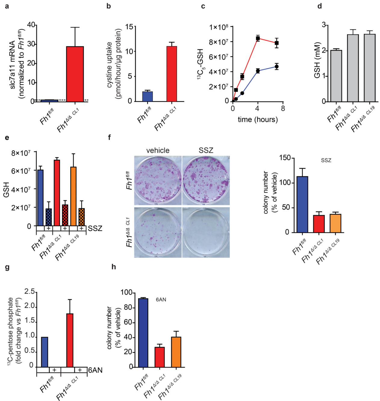
Figure 5. GSH succination triggers cystine uptake and GSH biosynthesis
