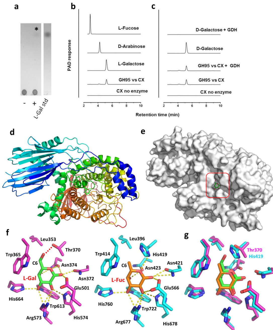
Figure 5. Activity and structure of BACOVA_03438 GH95 \alpha -L-galactosidase and comparison to the Bifidobacterium bifidum GH95 \alpha -L-fucosidase
