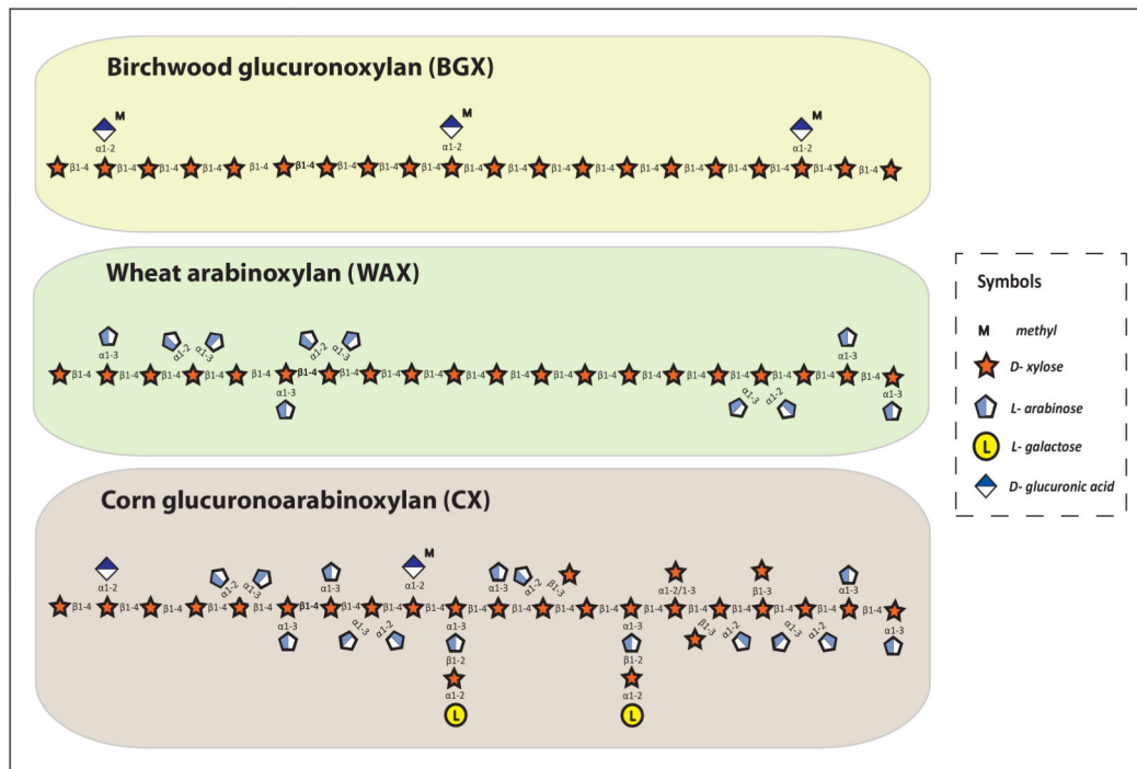
Figure 1. Schematic of the structures of the main classes of xylan
