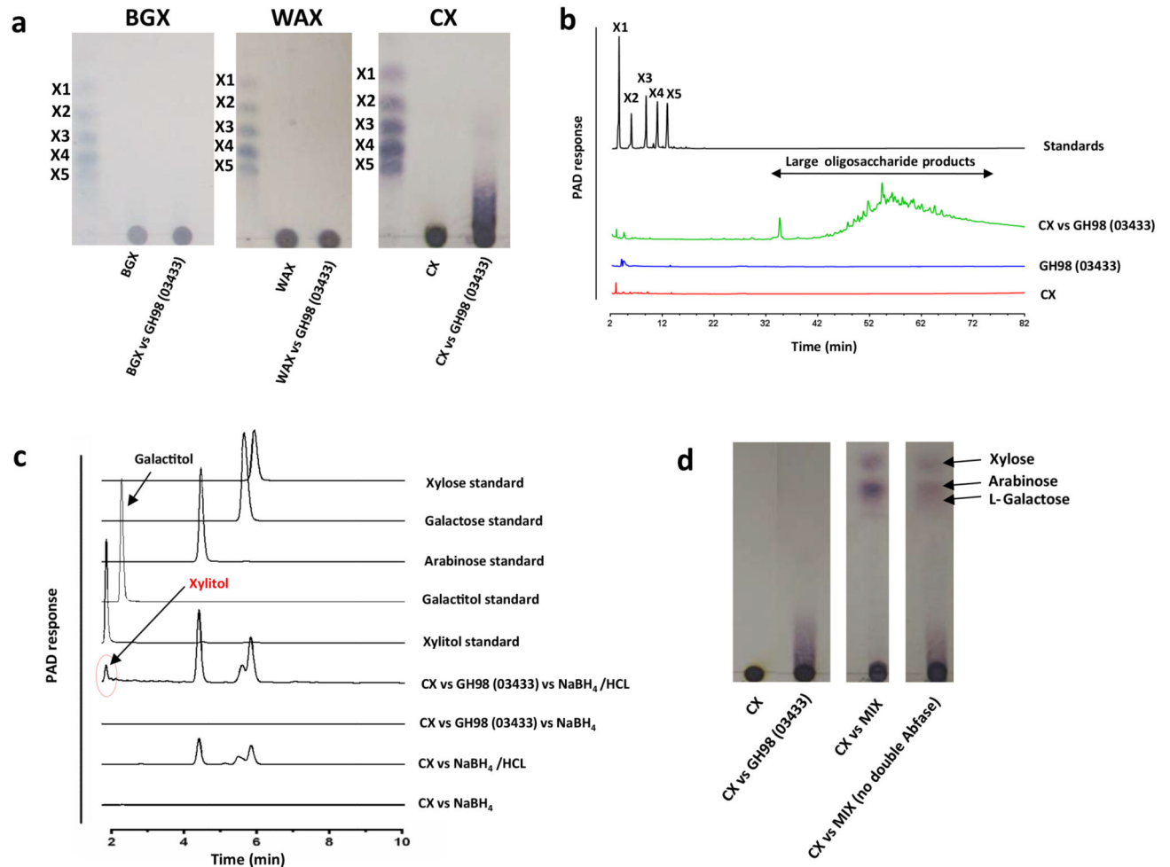
Figure 4. The activity of the GH98 enzyme BACOVA_03433
