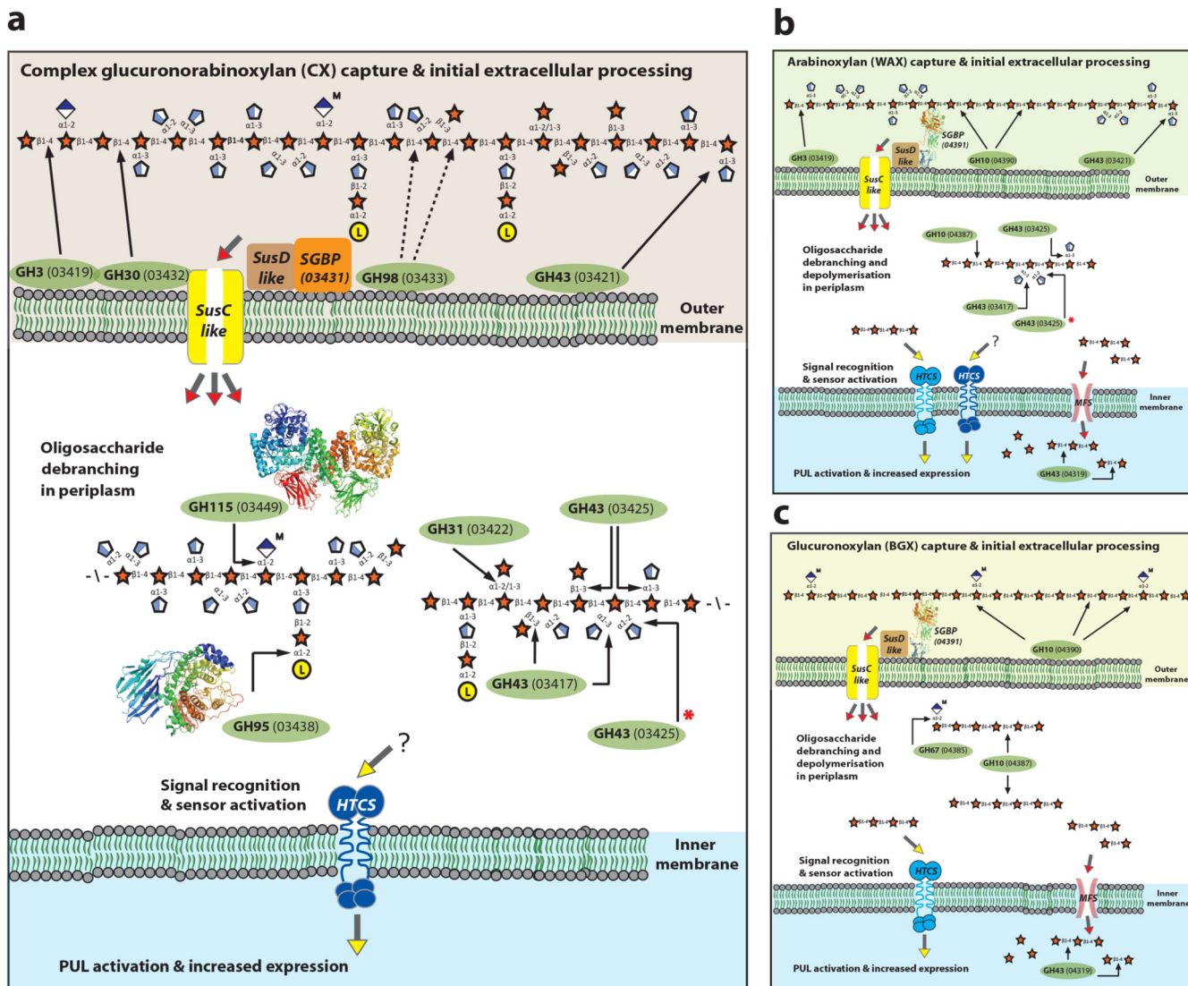
Figure 7. Models for the degradation of different forms of xylan by B. ovatus
