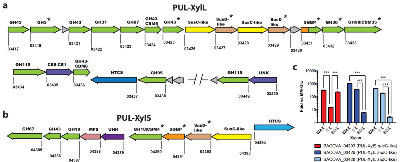
Figure 2. Schematic of the B. ovatus xylan PULs and differential expression during growth on different xylans
