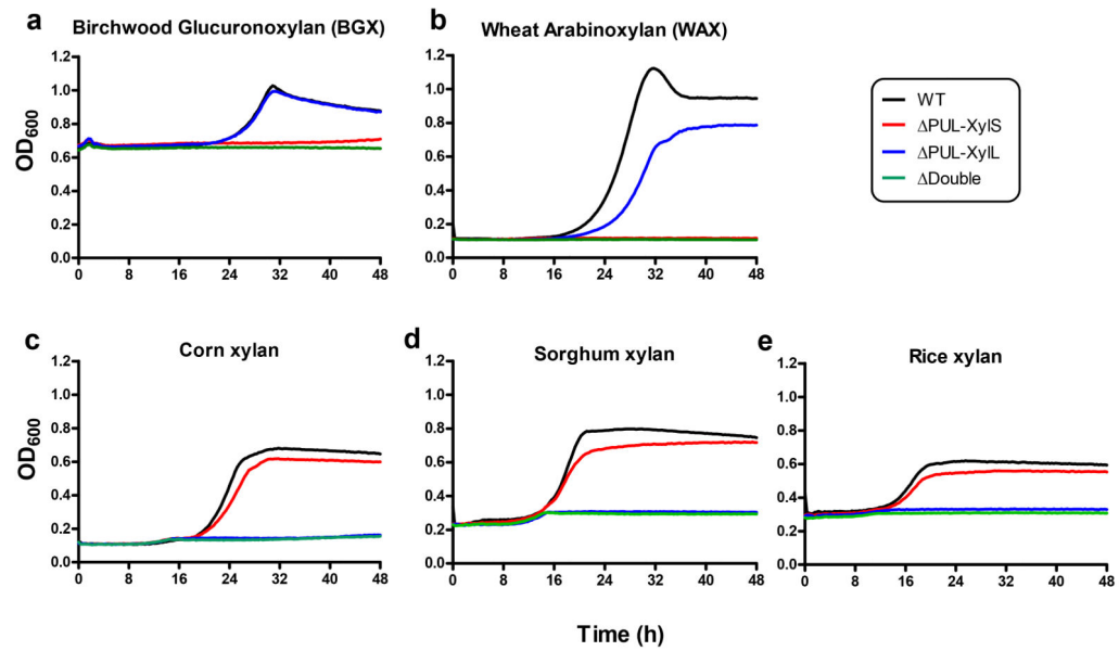
Figure 6. Growth profile of wild type and mutants of B. ovatus on xylans
