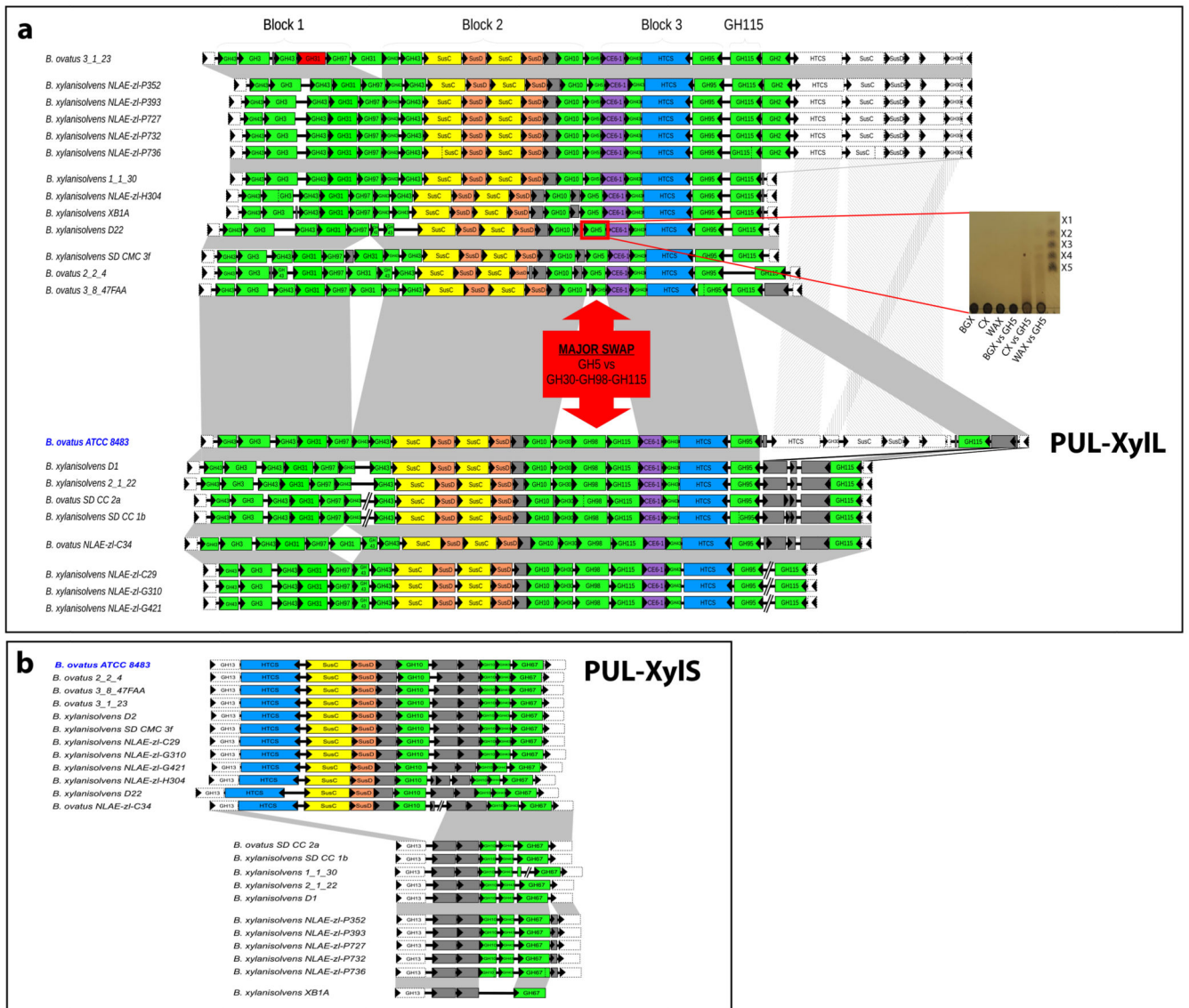
Figure 8. Conservation of the B. ovatus ATCC 8483 xylan PULs in other Bacteroides species CAZymes (green, CBM modules were omitted for clarity), susC -like (yellow), susD -like (orange) and the HTCS sensor-regulator (blue) genes are colour-coded. Genes encoding proteins of unknown function or non-CAZymes (e.g. surface glycan binding protein and MFS carbohydrate importer in PUL-XylIS) are shown in grey. a , PUL-XylL. Vertical dotted lines indicate split gene models, while missing gene models are shown in red. Microsyntenic segments are depicted by grey connectors, and include adjacent conserved non-PUL members (shown with dotted lines). Eighteen genes are conserved across all strains, and 17 of these form three highly conserved blocks indicated on top. The major difference between the two groups of the GH98 for GH5_21 swap is indicated. Inset shows a TLC of the activity of the recombinant B. xylanisolvens XBA1 GH5_21 enzyme (BXY_29320; boxed in red) against different xylans (1µM final enzyme vs 0.5% xylan in 20 mM sodium phosphate buffer, pH 7.0, 16 h at 37 °C). The B. xylanisolvens GH5 enzyme displays endo-xylanase
