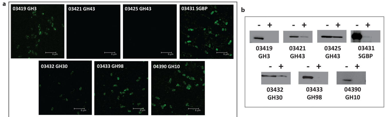
Figure 3. Cellular location of Xylan PUL enzymes containing a predicted N-terminal lipidation site or uncleaved transmembrane anchor
