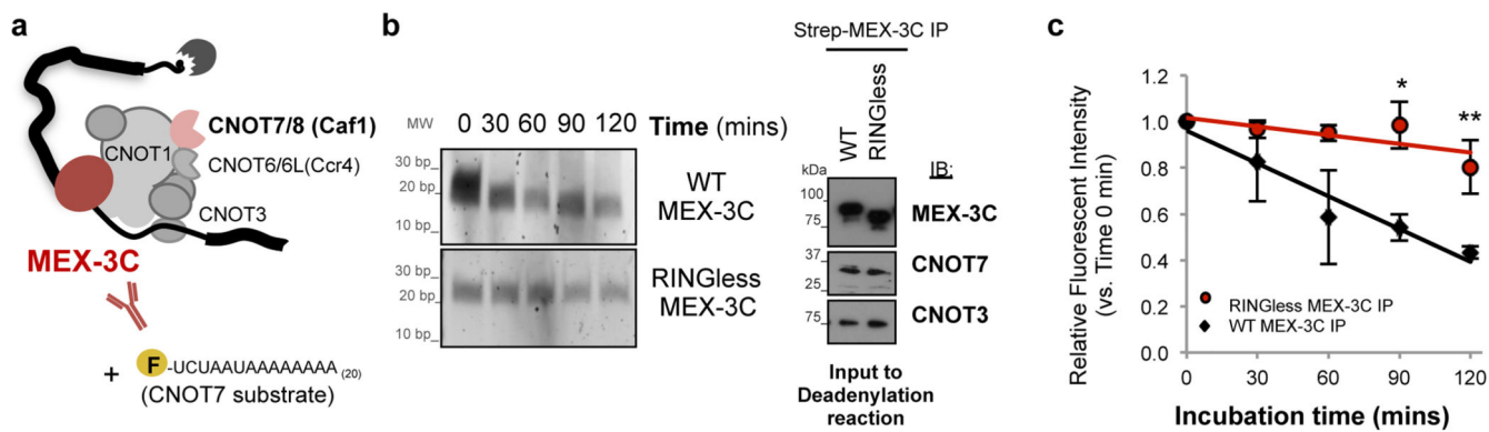
Figure 3. MEX-3C's E3 ubiquitin-ligase activity regulates deadenylation
