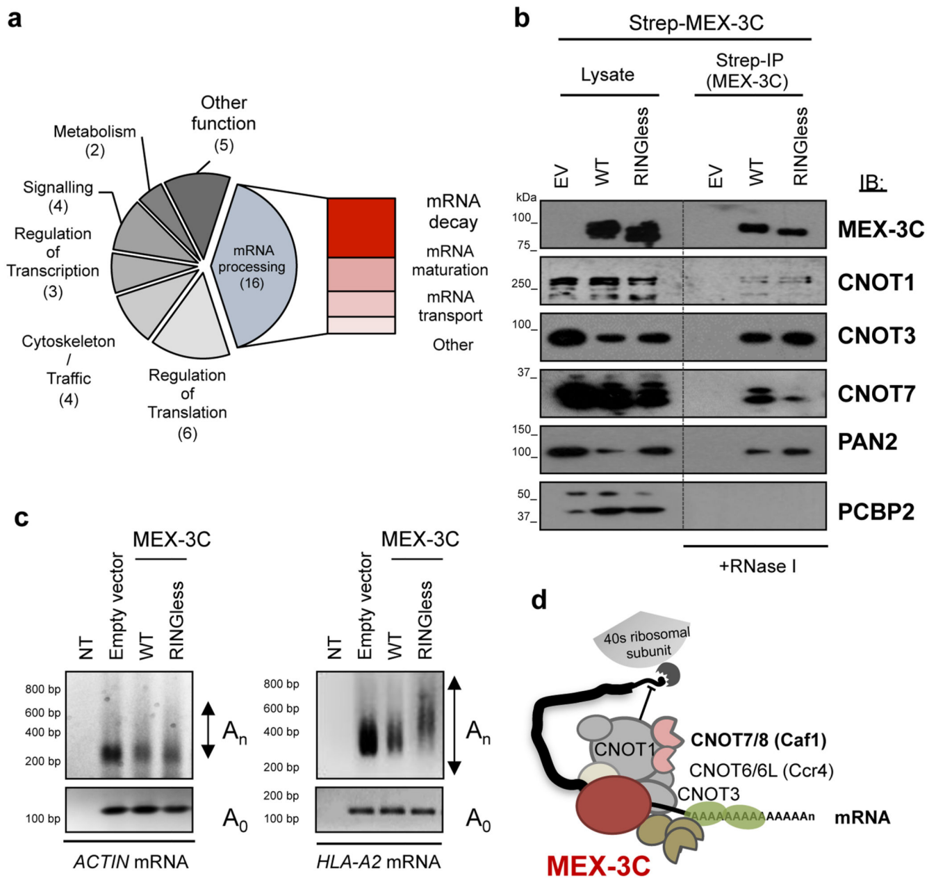
Figure 1. MEX-3C interacts with the major cytoplasmic deadenylation complexes and promotes the shortening of its target mRNA poly(A) tail through its ubiquitin ligase activity
