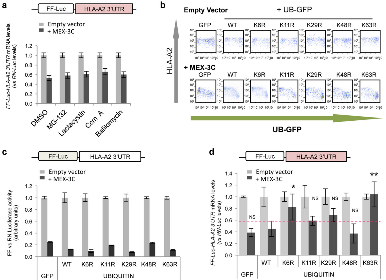
Figure 5. A non-proteolytic function for ubiquitin in the regulation of mRNA decay
