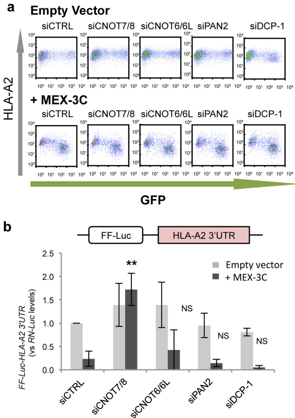
Figure 2. MEX-3C mediated degradation of FF-Luc-HLA-A2-3'UTR reporter mRNA is rescued by the depletion of CNOT7/8(Caf1), the major catalytic component of the CCR4-NOT deadenylation complex
