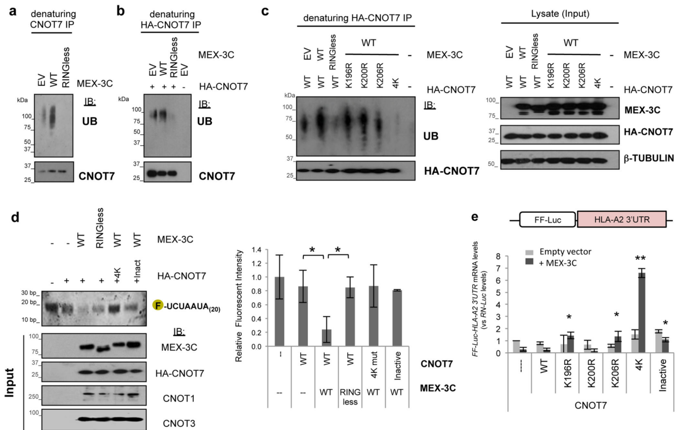
Figure 4. Ubiquitination of CNOT7 by MEX-3C is required for its deadenylation activity CNOT7 is ubiquitinated in-vivo in a MEX-3C dependent manner. Ubiquitin blots following denaturing immunoprecipitation (IP) of endogenous ( a ) or overexpressed ( b ) CNOT7. IB: Immunoblot. EV: Empty vector. (Supplementary Fig. 3a-b shows expression/loading controls.) c , Identification of the lysine residues in CNOT7 ubiquitinated by MEX-3C in-vivo . 4K-mutant: K196R,K200R,K203R,K206R. EV: Empty vector. d , Ubiquitination of CNOT7 by MEX-3C is required for its deadenylation activity. Deadenylation assay was performed as described in figure 3. *:P<0.05; unpaired Student's t -test. e , CNOT7 4K-mutant rescues MEX-3C mediated degradation of FF-Luc-HLA-A2-3'UTR reporter mRNA in-vivo . FF-Luc-HLA-A2-3'UTR mRNA levels were analysed as in Fig 2. CNOT7 catalytic inactive mutant (Inact): D40A/E42A. *: P<0.05 and **: P<0.005, both vs. wtCNOT7+ MEX-3C treatment; unpaired Student's t -test. Results are expressed as mean \pm SD of 3 independent experiments and relative to Empty Vector (EV) control. (Supplementary Fig. 4c shows expression/loading controls for this figure.)
