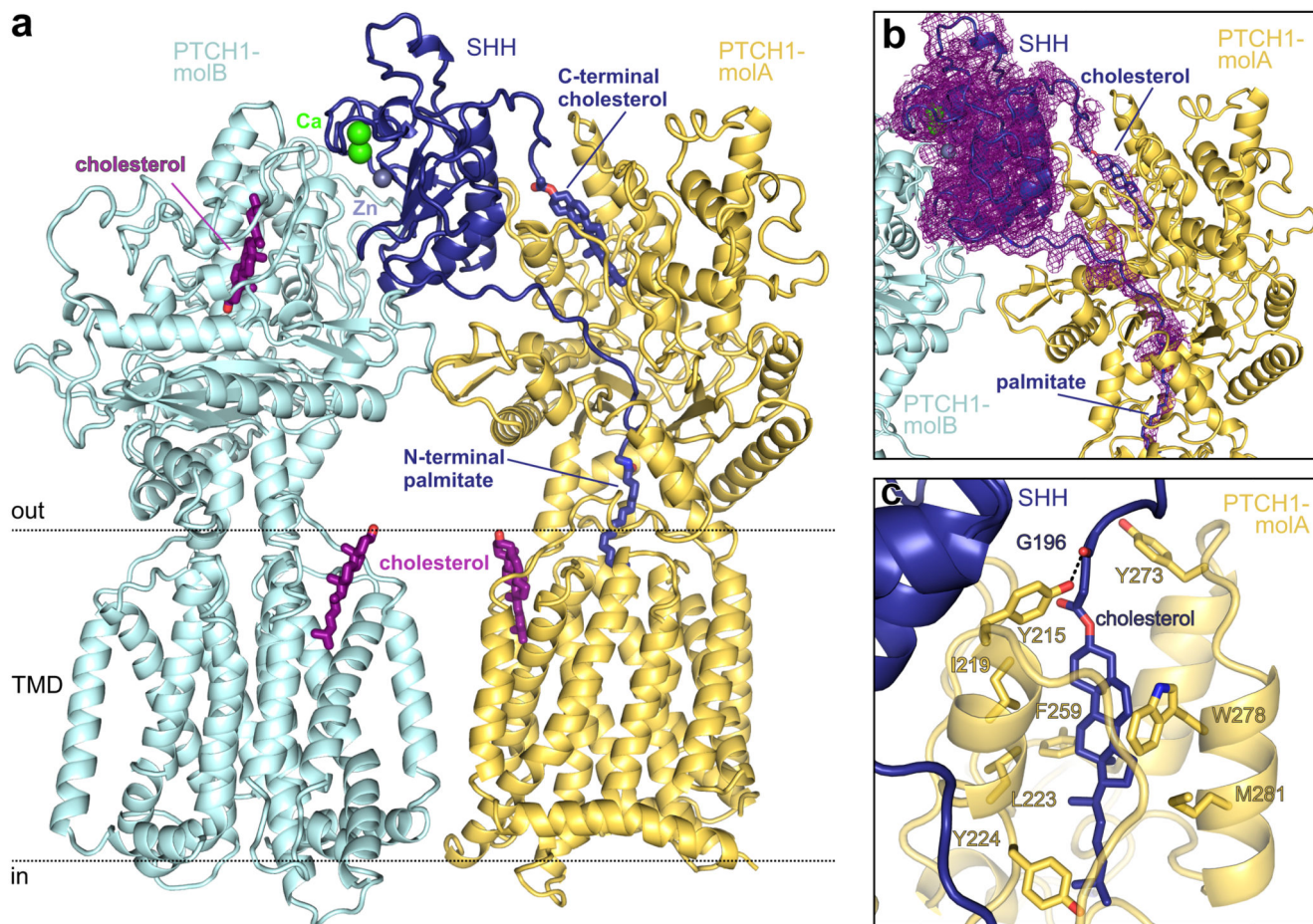
Figure 2. Structure of the PTCH1-pShhNc complex.
