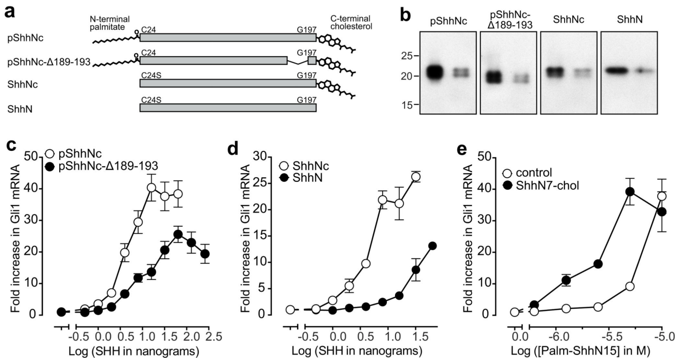
Figure 4. The cholesterol attached to pShhNc inactivates PTCH1.
