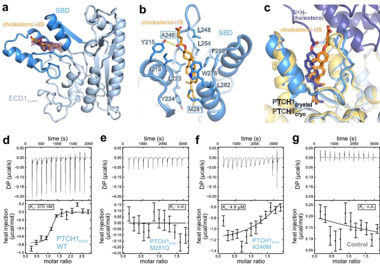
Figure 3. Structural and biophysical characterisation of the PTCH1 ECD-cholesterol complex. a , Crystal structure of the PTCH1 ECD1 -cholesterol-hemisuccinate (cholesterol-HS) complex, with the 3-helix SBD coloured dark blue. The initial 2Fo-Fc map at 1.0 \sigma and 1.9 Å resolution before inclusion of cholesterol-HS is shown in wire representation. b , Close-up view of the sterol-binding site with cholesterol-HS depicted in orange sticks. c , Superposition of the PTCH1 ECD1 -cholesterol-HS crystal structure on the improved PTCH1-pShhNc cryo-EM structure. The entrance of the sterol-binding pocket is slightly rearranged, likely due to different steric constraints of the hemisuccinate group compared to the glycine ester linkage found in pShhNc. d-g , Raw ITC data (upper panel) and binding isotherms (lower panel) for titration of PEG-cholesterol into solutions containing PTCH1 ECD1 -WT ( d ), PTCH1 ECD1 -M281Q ( e ) and PTCH1 ECD1 -A246M ( f ). PEG200, unconjugated to cholesterol, was titrated into a PTCH1 ECD1 -WT solution as a control ( g ). Curves show the A + B \rightleftharpoons AB binding model that was used for local fitting to the data. The K_d is shown where it could be calculated. Bars shown on the isotherm reflect errors associated with integration of the injection peaks in the corresponding thermograms (68% confidence around extrapolation of pre- and post-injection baselines).
