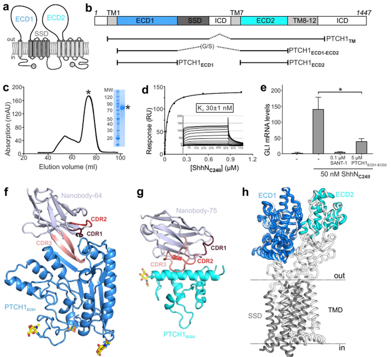
Figure 1. Structural and function characterization of PTCH1-nanobody interactions.
