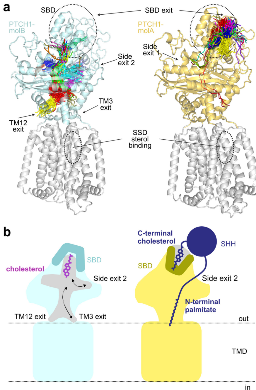
Figure 6. Tunnel analysis of PTCH1 structures.
