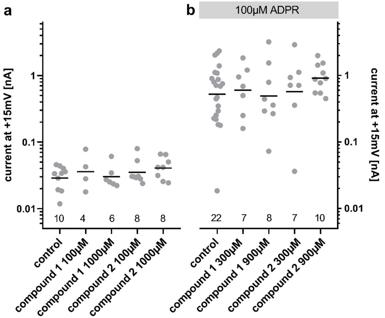
Figure 3. Effect of 1 and 2 on whole cell currents in hTRPM2 expressing HEK293 cells.
