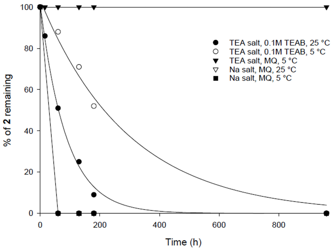
Figure 2. Stability of compound 2 under various aqueous conditions
