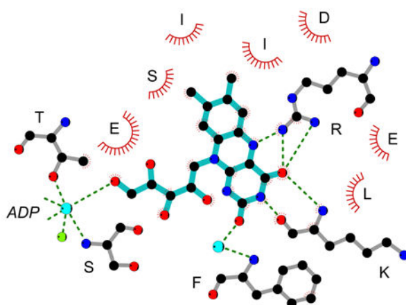
riboflavin kinase (protein)
