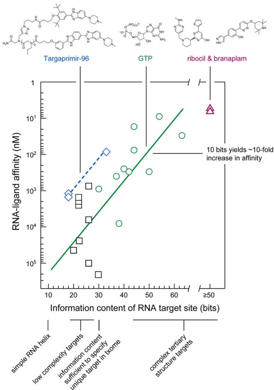
Figure 6: Relationship between information content and specificity and binding affinity. Solid and dashed lines show the relationship between RNA target information content and binding affinity for GTP (circles) and Targaprimir-96 (diamonds) (based on data from refs. 73,78). Simple helices are assigned 9 \pm 2 bits of information. Ribocil 30 and branaplam 32 are estimated to have 50 bits of information and are placed on a separate scale. Binding data for medium-complexity targets (squares) are from the following: influenza A promoter stem-loop (20 bits) 49 , TAR (22 bits) 37,39,40,48 , HCV IRES bulged-stem (26 bits) 36,41,102 , and SARS pseudoknot (30 bits) 47,101 .
