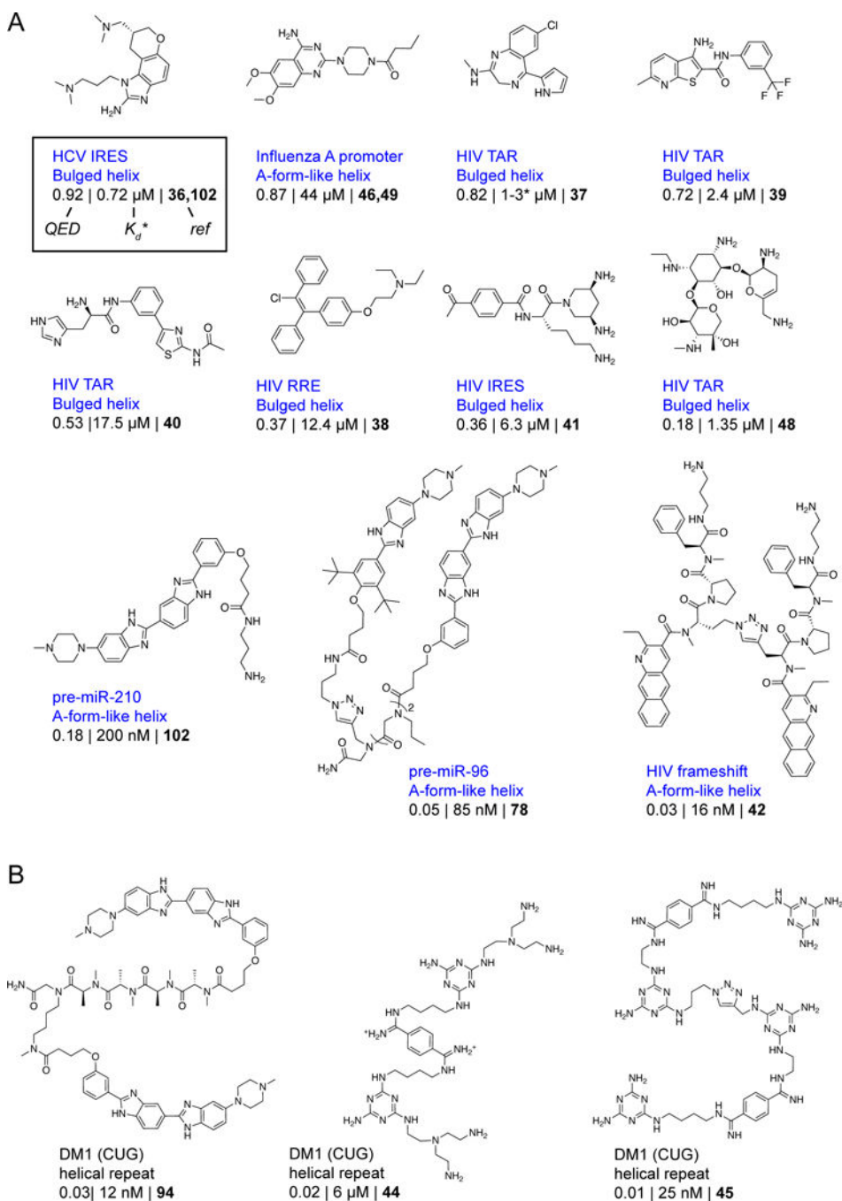
Figure 3: Instructional examples of bioactive small molecules that bind RNA secondary structures.
