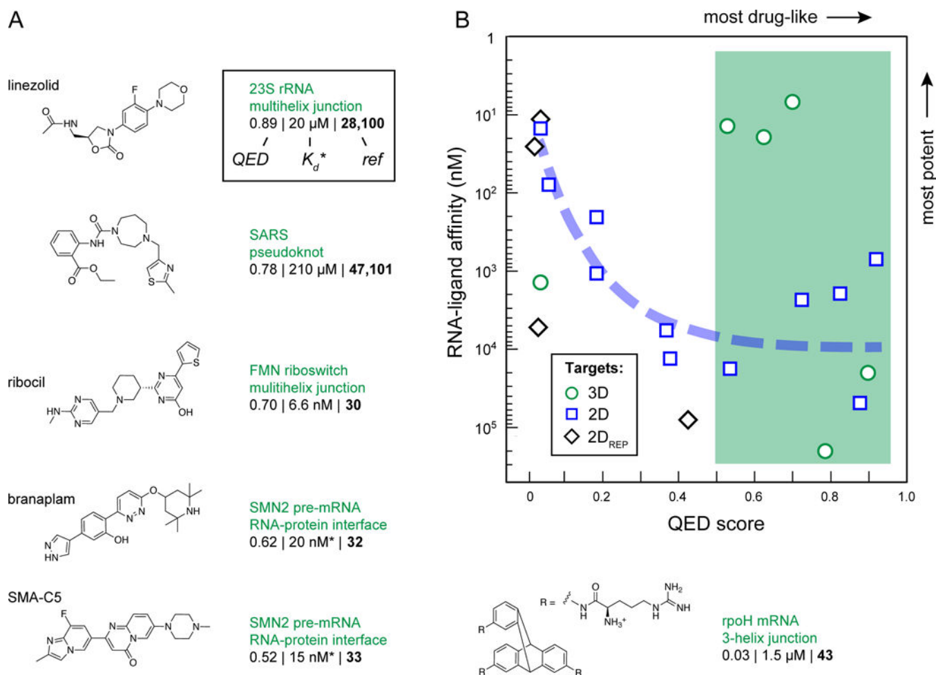
Figure 2: Instructional examples of bioactive small molecules that bind to RNA.
