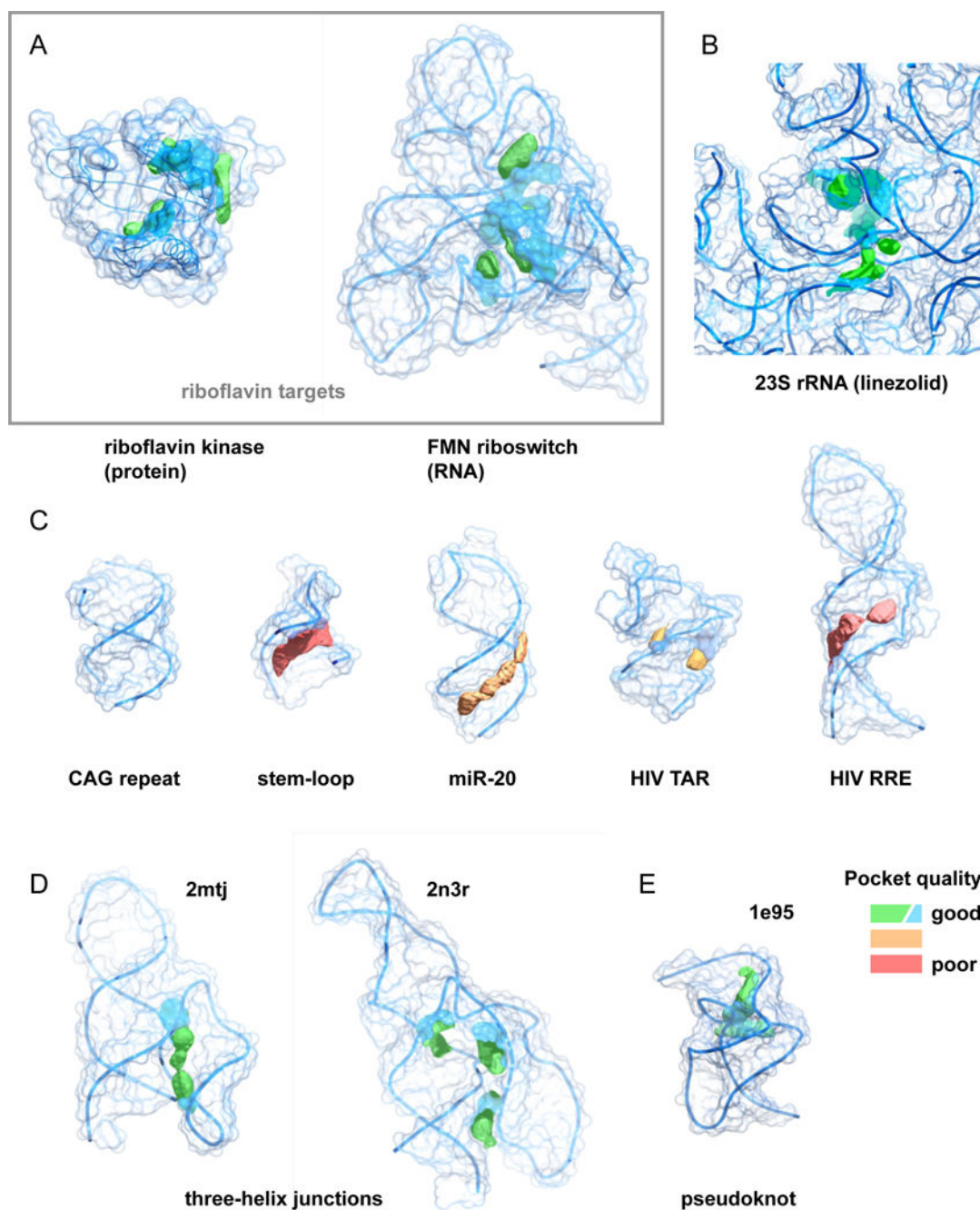
Figure 7: Pocket analysis for current and aspirational RNA targets.
