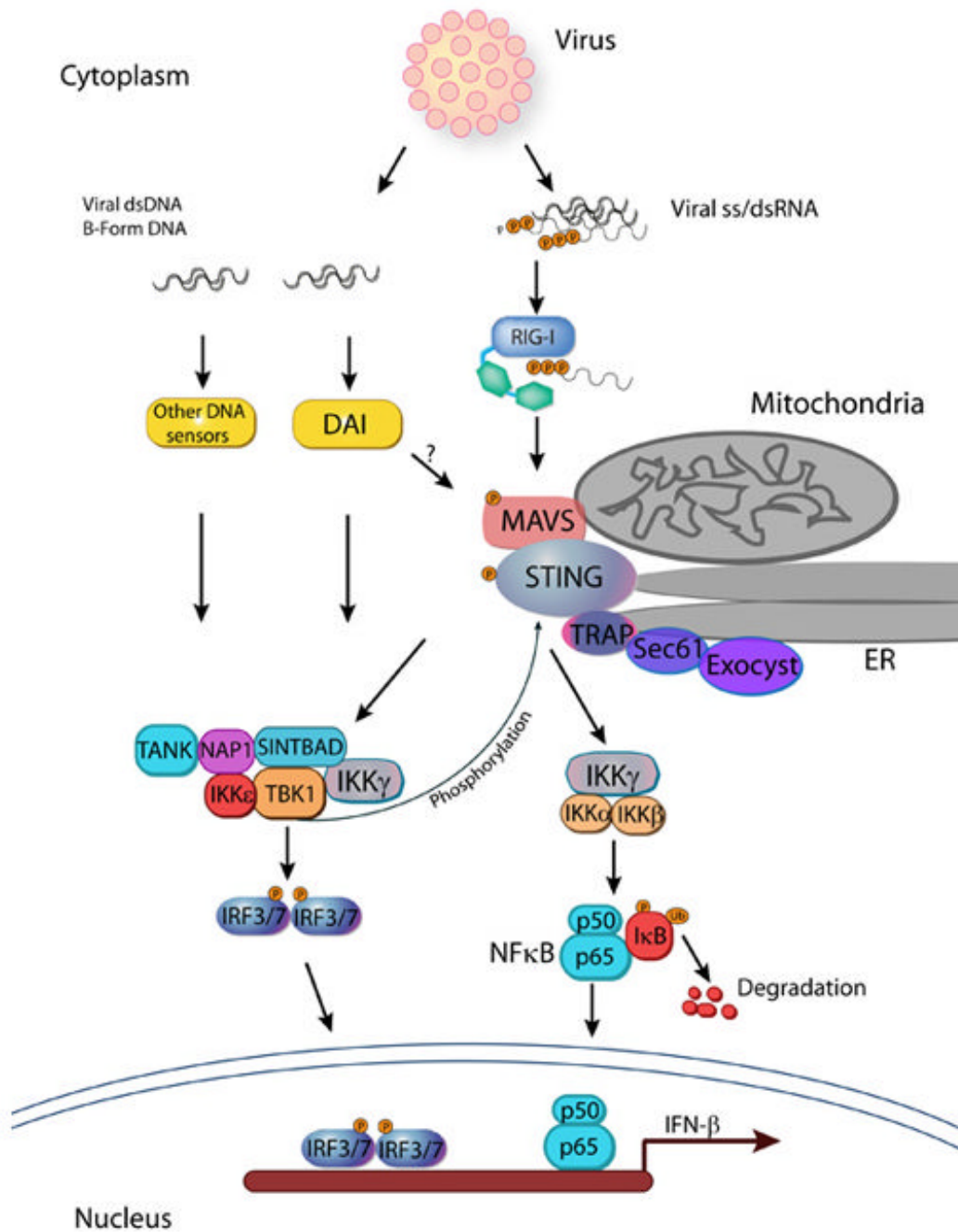
Figure 1. Cytoplasmic recognition of viral nucleic acids
