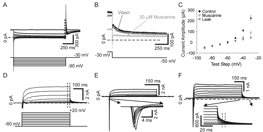
Fig. 7. Voltage-clamp protocols used to examine four currents in sympathetic neurons
