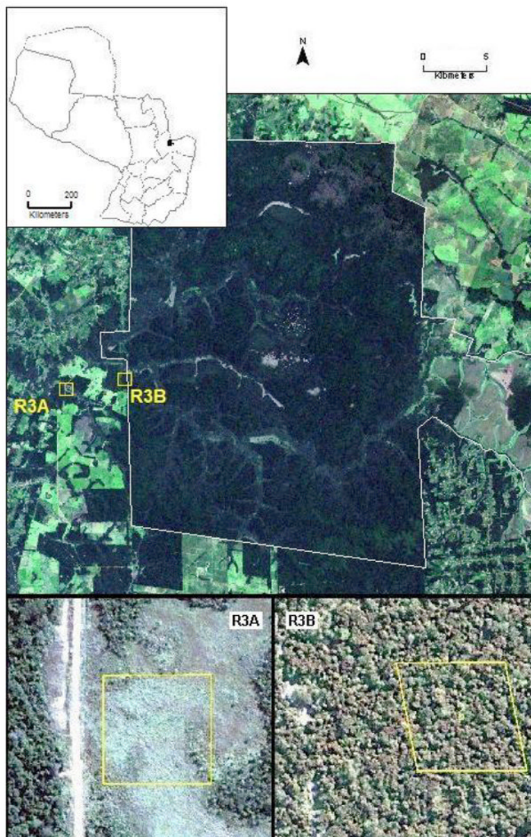
Figure 1. Natural color satellite imagery showing location and general land cover characteristics of the two data collection grids. Larger image (acquired Feb. 2003 from Landsat ETM+), shows the general setting of the collection grids within and near the Mbaracayú forest reserve (reserve boundaries are indicated by the white outline). Smaller images (acquired May 2005 from DigitalGlobe Quickbird) show detailed views of the forested (R3B) and deforested (R3A) sites. Boxes indicate the exact boundaries of the 1 ha trapping grids. Location of the study site within Paraguay is indicated by the inset map.
