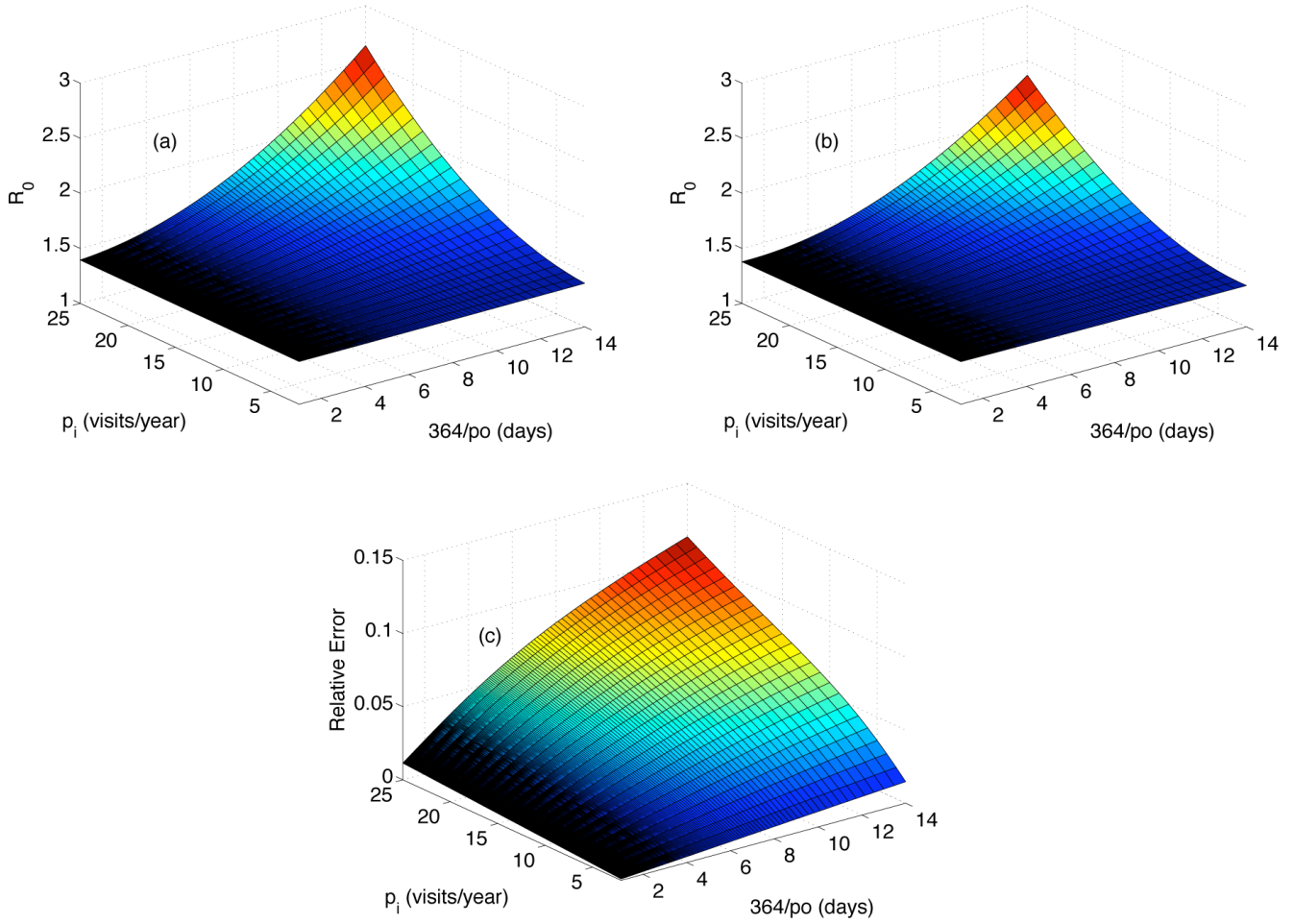
Figure 7. The basic reproduction number \mathcal{R}_0 for the habitat-based model (3.4)–(3.6) as a function of the average number of visits to boundary region ( p_i ) and average length of time (days) spent in the boundary region ( 364/p_o ), (a) based on formula (4.12), [Approx], and (b) based on the parameter values in Table 1, [Exact]. The graph in (c) is the relative difference or relative error in these two \mathcal{R}_0 values: ([\text{Approx}] - [\text{Exact}]) / [\text{Exact}] .
