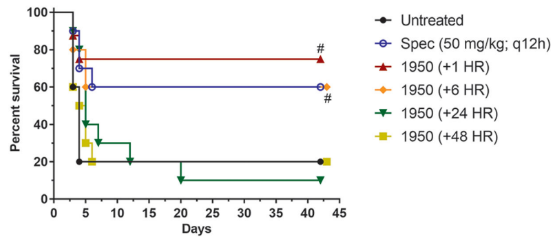
Fig. 4. Survival of BALB/c mice infected i.n. with 2 \times 10^4 CFU B. mallei FMH. Treatment with 1950 ( 50 \text{ mg kg}^{-1} , BID) was initiated at 1, 6, 24, or 48 h post-infection and was administered s.c. for 14 days. Control mice were treated with saline (untreated) or spectinomycin ( 50 \text{ mg kg}^{-1} , BID) starting at 1 h post-infection. 1950 (1 h) group: n = 8 ; all other groups: n = 10 . # Significantly different from untreated control group ( P < 0.05 ).
