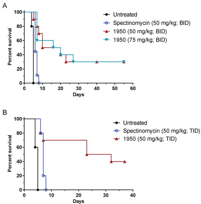
Fig. 5. Effect of compound 1950 on F. tularensis infection. (A) Survival of mice ( n = 10 ) infected i.n. with 1 \times 10^3 CFU F. tularensis strain SchuS4 ( 10 \times LD_{50} ). Treatment with saline (untreated), spectinomycin ( 50 \text{ mg kg}^{-1} , BID), or 1950 ( 50 or 75 \text{ mg kg}^{-1} , BID) administered s.c. started at 1 h post-infection and continued for 14 days. Mice were monitored for morbidity and mortality for 55 days. # Significantly different from untreated control ( P = 0.0001 ) and spectinomycin control ( P = 0.0013 ). (B) Survival of mice infected i.n. with 900 CFU F. tularensis strain SchuS4 ( 10 \times LD_{50} ). Treatment with saline (untreated), spectinomycin ( 50 \text{ mg kg}^{-1} , TID), or 1950 ( 50 \text{ mg kg}^{-1} , TID) administered s.c. was initiated at 1 h post-infection and continued for 14 days. Mice were monitored for morbidity and mortality for 37 days. # Significantly different from untreated control ( P < 0.0001 ) and the spectinomycin control mice ( P = 0.0315 ).
