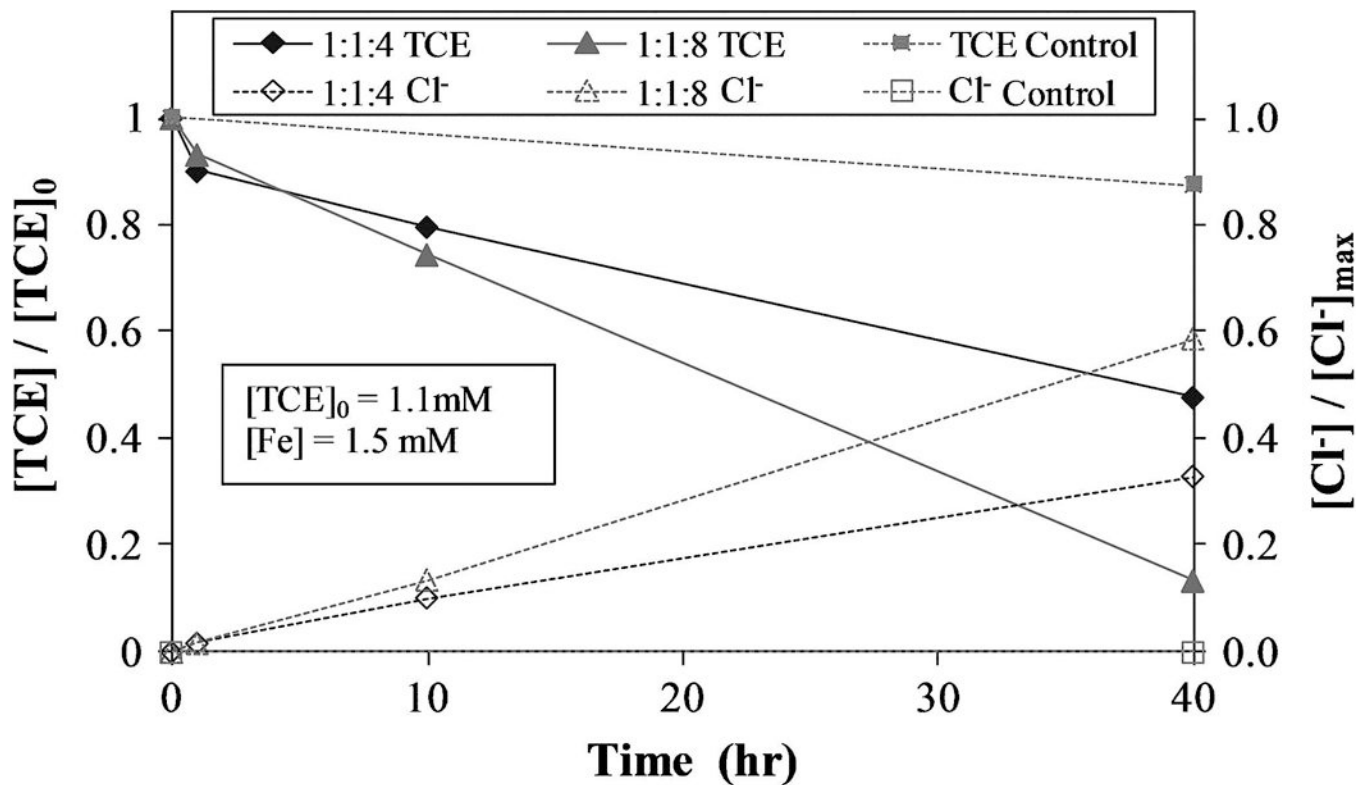
FIG. 6. TCE reacted and Cl - formed for varying Fe(II): L:H 2 O 2 molar ratio with initial TCE concentration of 1.1mM, where L is citrate. Conducted in natural water obtained from the DOE site. Control experiment conducted without H 2 O 2 . Initial pH = 7.
