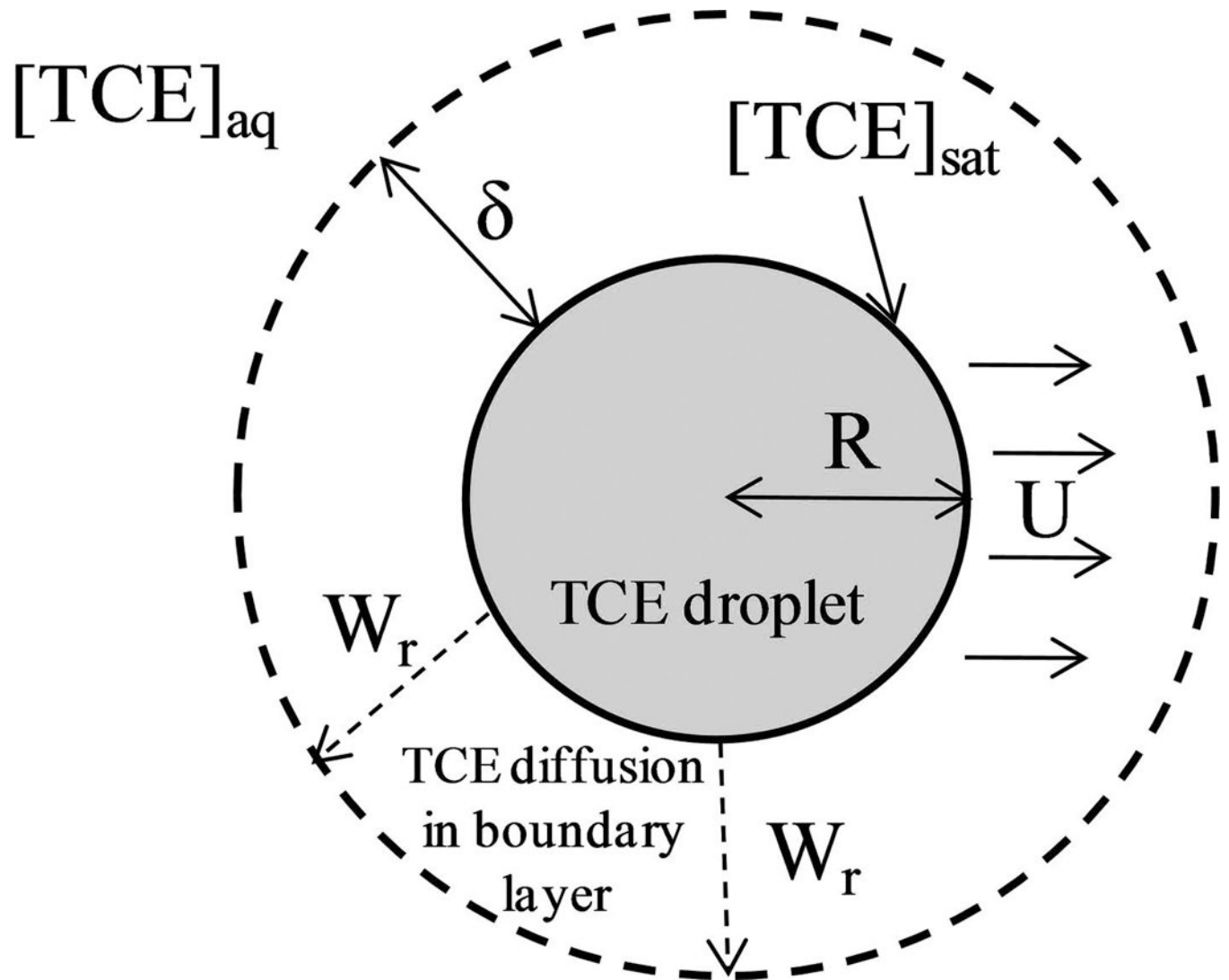
FIG. 10. Schematic of TCE droplet dissolution into aqueous solution.
