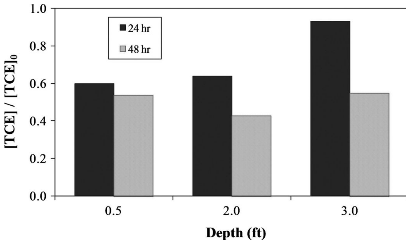
FIG. 15. TCE dechlorination results for RGA packed column. [TCE]_0 = 0.41\text{mM} , [Fe] = 1.5\text{mM} , [L]:[Fe] = 1:1 . H_2O_2 injections at 0 and 24 h for 2:1 [H_2O_2]:[Fe] molar ratio. Column flowrate = 2.5 ft/day. (\text{mol } Cl^- \text{ formed})/(\text{mol TCE reacted}) \approx 3 (not shown in figure).
