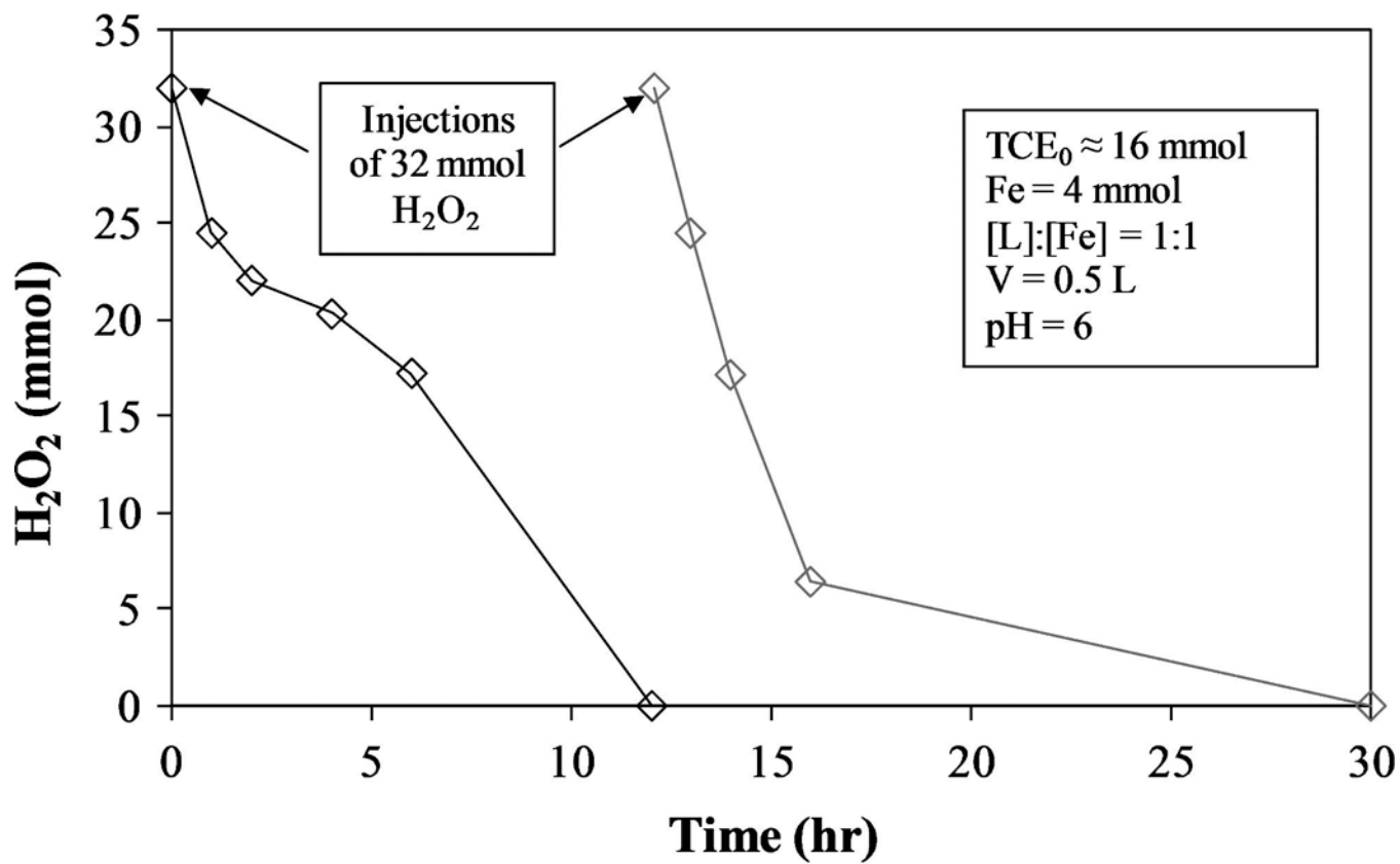
FIG. 11. \text{H}_2\text{O}_2 degradation profile for chelate-modified Fenton reaction in two-phase TCE system. \text{H}_2\text{O}_2 injected at time = 0 and 12 h.
