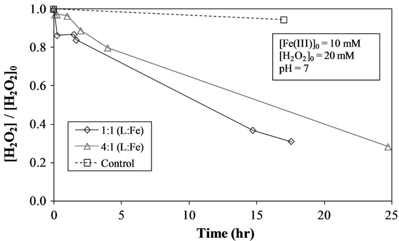
FIG. 5. Role of ferric iron (Fe(III)) on \text{H}_2\text{O}_2 decomposition with varying [L]:[Fe] molar ratio. L = citrate.
