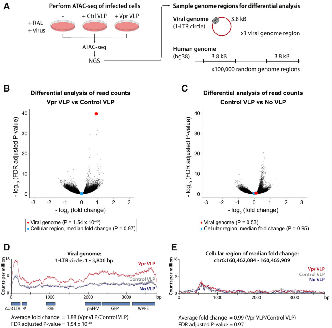
Figure 6. The SMC5/6 complex induces compaction of unintegrated lentiviral genomes (A–E) ATAC-seq shows increased unintegrated virus chromatin accessibility upon Vpr-mediated SLF2 depletion. (A) WT Jurkat cells were co-infected with a GFP reporter lentivirus and control or Vpr VLPs in the presence of RAL, and ATAC-seq performed 48 hpi. Reads were aligned to the human and viral 1-LTR circle reference genomes. To quantify effects on chromatin accessibility, 100,000 cellular genome regions of equal size to the viral genome (3.8 kB) were randomly defined, and the fold change in normalized sequence coverage between conditions calculated for each region, viral or cellular. For each data point, significance was determined using Fisher’s t test, adjusted by FDR to correct for multiple testing. Comparisons were visualized as volcano plots summarizing data for all 100,000 cellular regions and the viral genome (plotting regions with >50 aligned reads): (B) comparing data for Vpr VLP with control VLP and (C) comparing data for control VLPs with No VLPs. The viral genome (red) and the cellular region of median fold change (blue) are highlighted as enlarged data points for each comparison. Normalized read density for the viral genome is displayed in (D) and for a representative cellular region of median fold change in (E).
