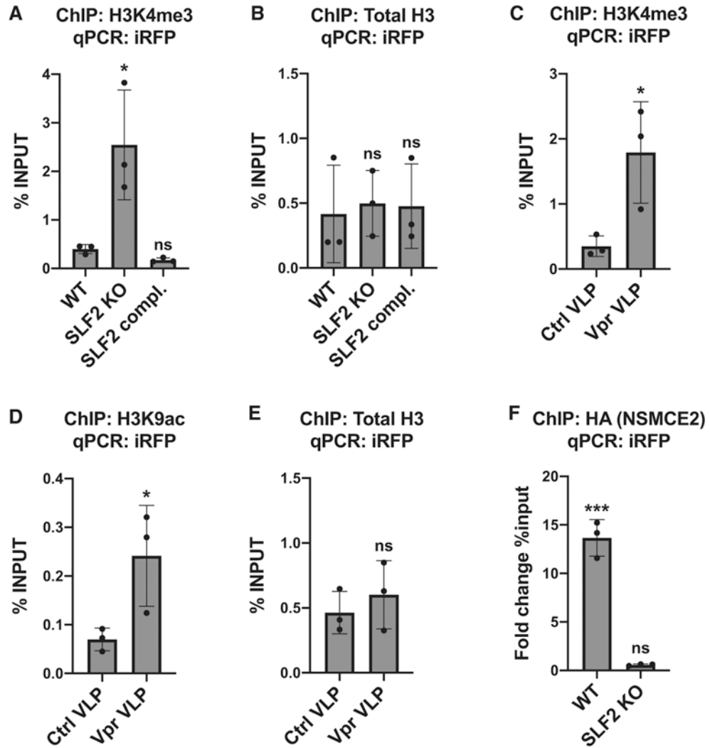
Figure 5. The SMC5/6 complex is recruited in an SLF2-dependent manner to unintegrated lentiviral genomes leading to a loss of H3K4me3 and H3K9ac on viral chromatin (A and B) Knockout of SLF2 increases H3K4me3 on unintegrated virus. WT, clonal SLF2 KO and SLF2 complemented SLF2 KO cells were infected with SFFV-iRFP lentiviral reporters in presence of RAL. 48 hpi, ChIP was performed using antibodies against (A) H3K4me3 and (B) total H3. qPCR data from each ChIP experiment were calculated as the percentage of input DNA. Histograms summarize data from n = 3 experiments. (C–E) Vpr-mediated depletion of SLF2 increases H3K4me3 and H3K9ac on unintegrated virus. WT cells were co-transduced with iRFP reporters and either control or Vpr VLPs in presence of RAL. 48 hpi, ChIP was performed using antibodies against (C) H3K4me3, (D) H3K9ac, and (E) total H3, calculated as the percentage of input DNA ( n = 3 ). (F) The SMC5/6 complex binds unintegrated viral genomes via SLF2. WT or SLF2 KO cells expressing 3xHA-NSMCE2 were infected with SFFV-iRFP in presence of RAL. 48 hpi, ChIP was performed using antibodies against the HA-tag. Data were calculated as the fold change in percentage of input DNA compared with a matched control ChIP experiment
