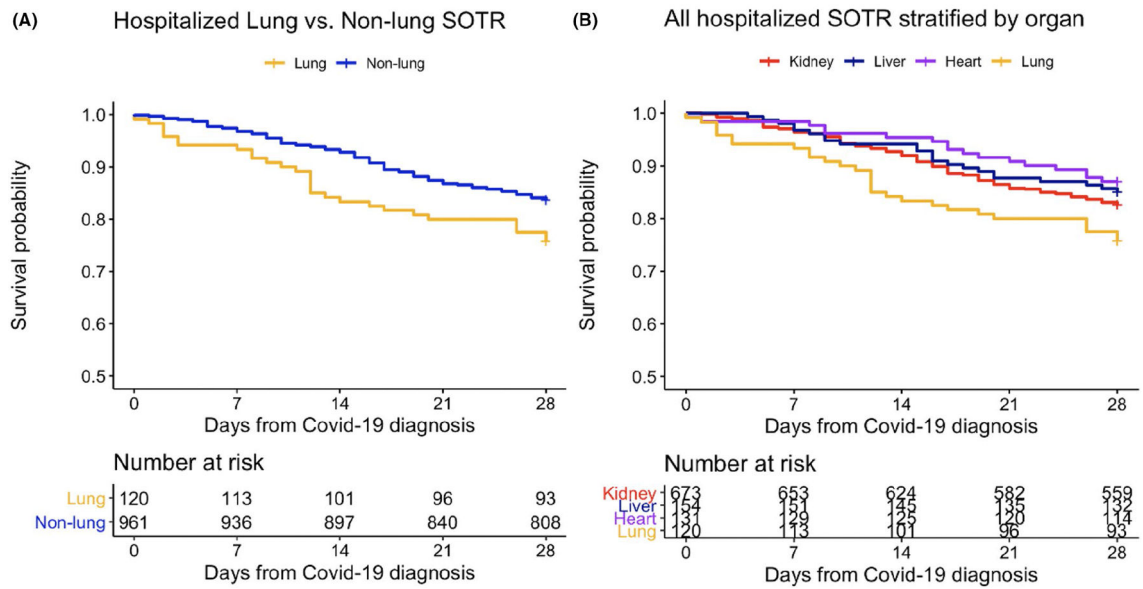
FIGURE 1. Unadjusted Kaplan–Meier curves for all-cause mortality within 28-days after COVID-19 diagnosis for hospitalized solid organ transplant recipients. Abbreviation: solid organ transplant recipients (SOTR). Note: Lung includes 1 lung/liver and 2 heart/lung recipients. Heart includes 14 heart/kidney and 1 heart/kidney/small bowel recipients. Liver includes 33 liver/kidney, 2 liver/pancreas/small bowel. Kidney includes 17 kidney/pancreas recipients. Recipients of other organs (1 vascular composite allograft and 2 small bowel recipients) not included
