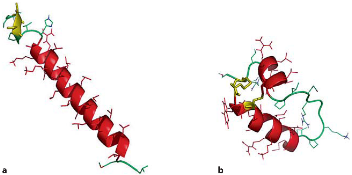
Fig. 1. a Molecular graphics illustration of SP-C33 in methanol based on the structure of native porcine SP-C (1SPF). Helical residues in the transmembrane sequence are in red, the N-terminal serine residues are in yellow, and disordered segments are in green. b Mini-B structure in methanol based on the structure of Mini-B (1SSZ) with the helical segments in red, the engineered loop in green and the disulfide linkages in yellow.
