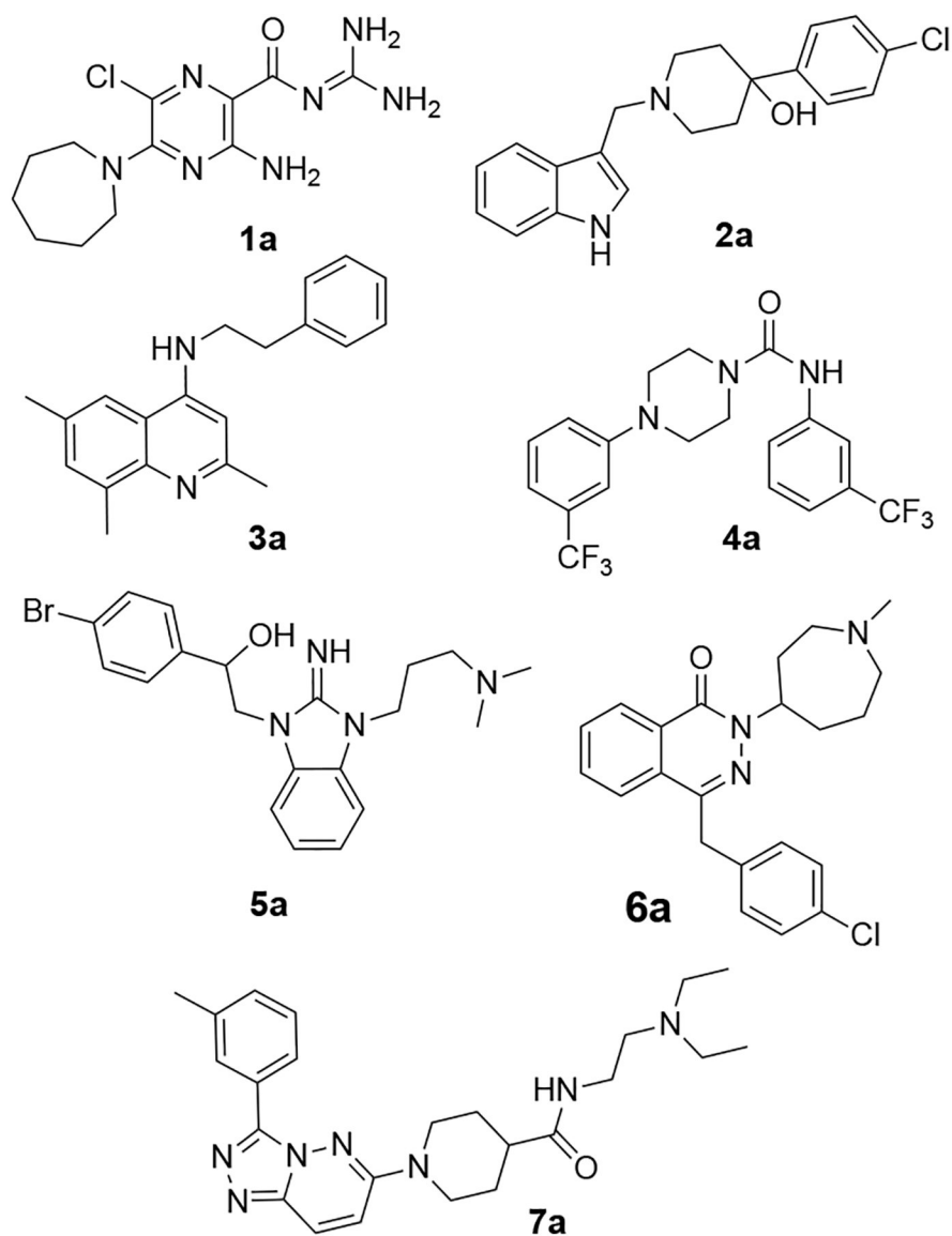
Figure 3. Hit compounds resulting from HTS campaign.
