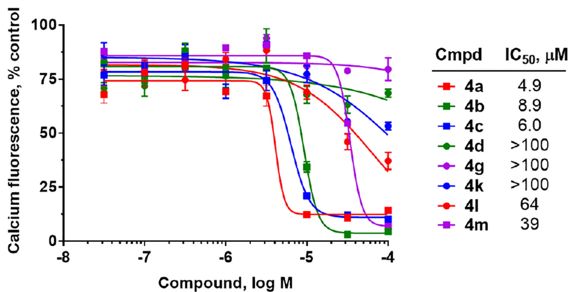
Figure 5. Inhibition of progesterone-induced calcium uptake in human sperm by selected analogs in hit series 4. Data presented as the mean of 3 independent experiments (except 4m , n=2) with error bars representing the SEM.
