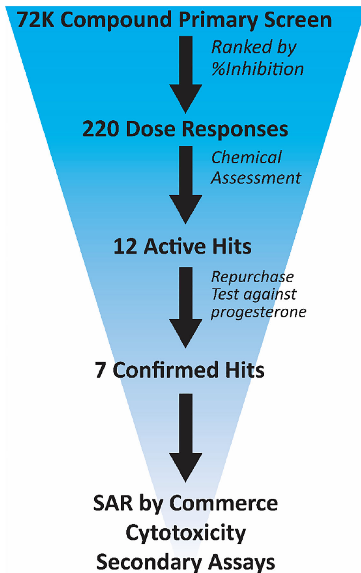
Figure 2. Graphical representation of HTS workflow.
