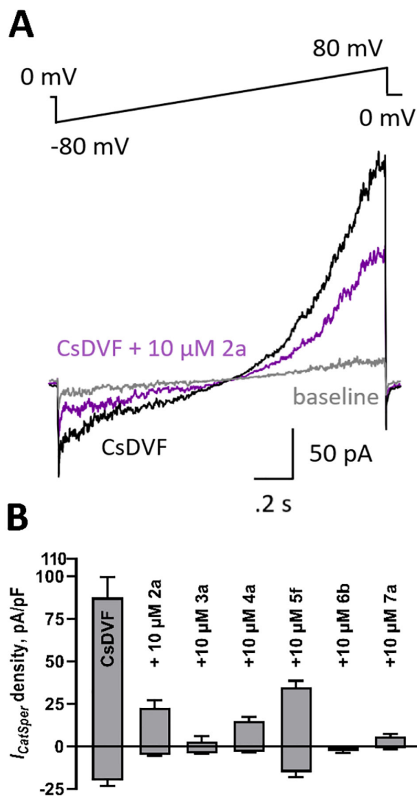
Figure 7. Inhibition of human I_{CatSper} by compounds from each hit series. A. Representative I_{CatSper} recording from human sperm in cesium divalent free media (CsDVF) elicited by the voltage ramp in the absence (black) and presence (purple) of test compound 2a . Baseline signal in high saline (HS) buffer shown in grey. B. Current density plots of tested compounds showing inhibition of I_{CatSper} at +80 mV (positive scale) or -80 mV (negative scale). Data are displayed as means \pm SEM of at least 3 independent experiments.
