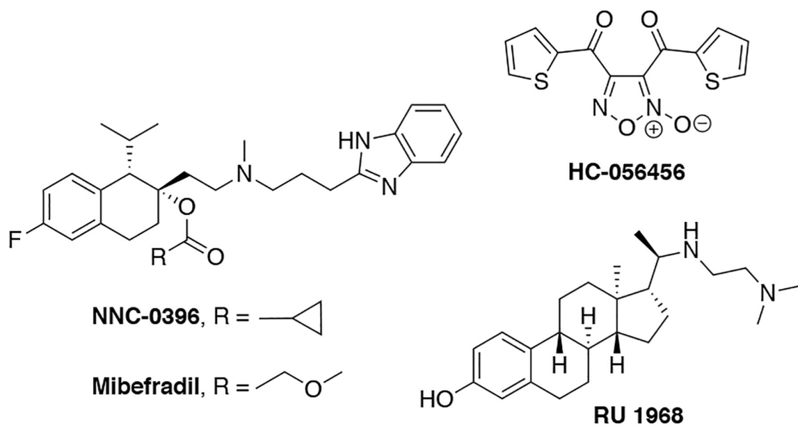
Figure 1. Structures of known CatSper inhibitors.
