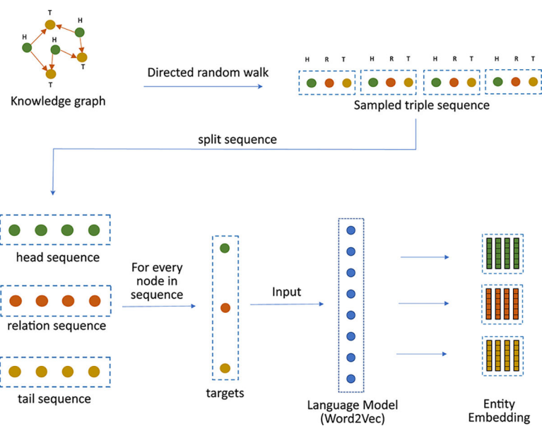
Fig. 5. TripleWalk model
