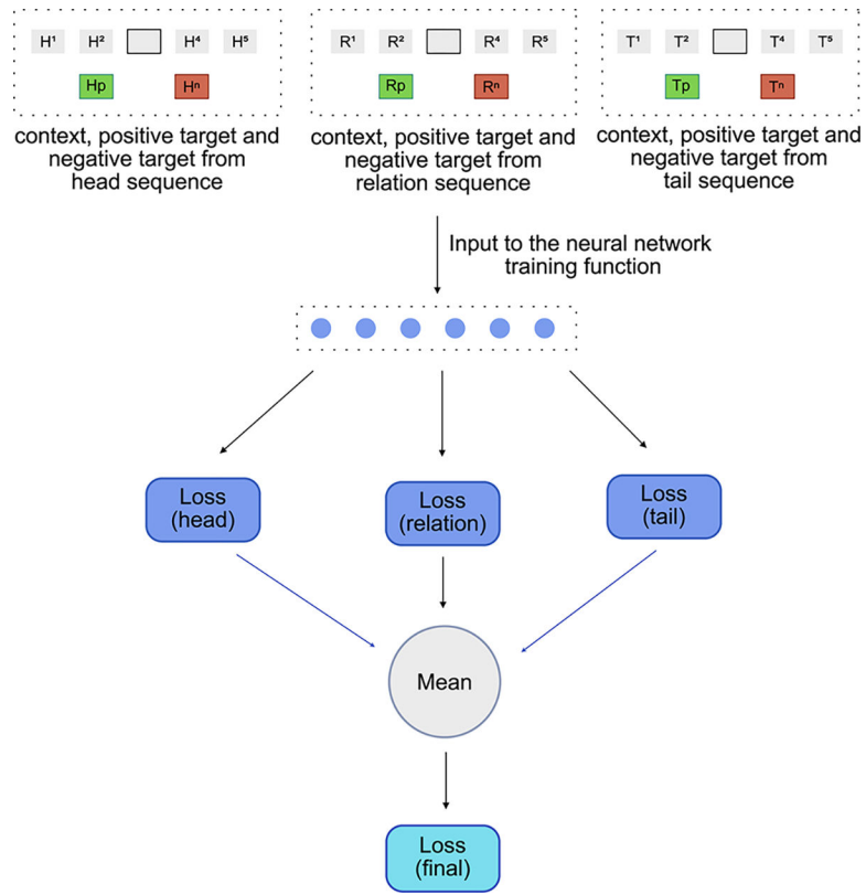
Fig. 6. Modified Word2Vec model
