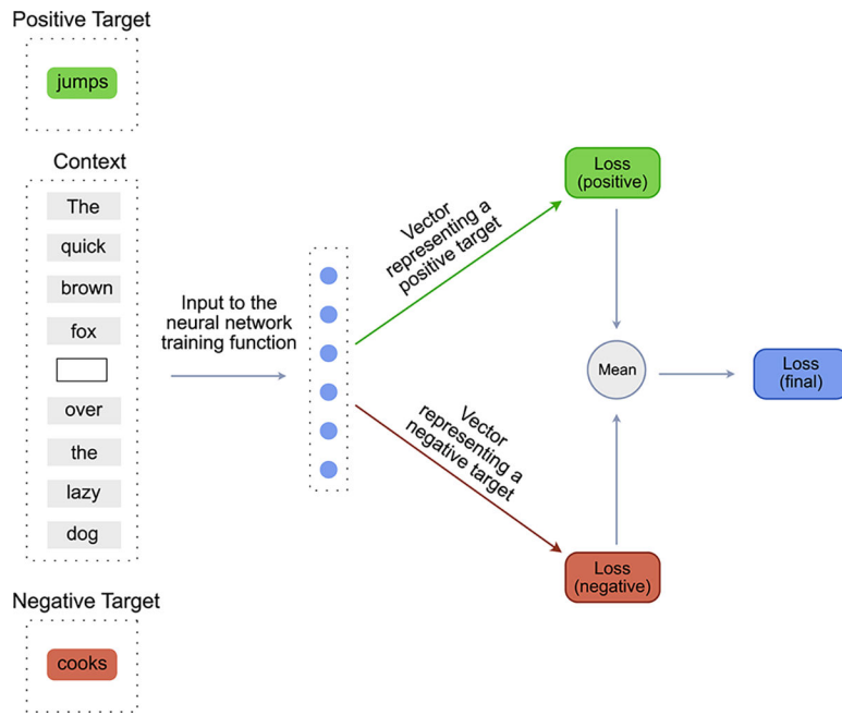
Fig. 2. Word2vec model (CBOV) that predicts the target word given the context.
