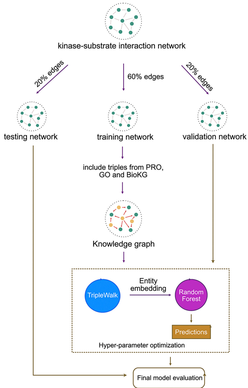
Fig. 8. TripleWalk model training and hyperparameter optimization
