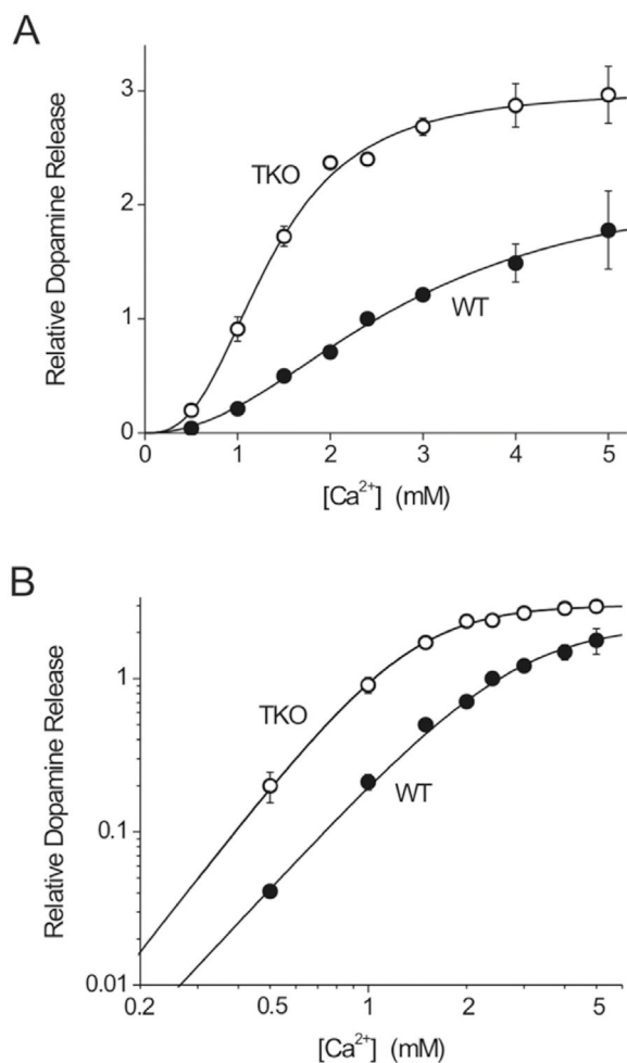
Figure 5. Calcium dependence of DA release in striatal slices. A) Relative [DA]_{\max} for TKO and WT animals at 0.5–5 mM extracellular [Ca^{2+}] . TKO animals release significantly more DA at all [Ca^{2+}] . B) Log-plot used to determine stoichiometric relationship between DA release and [Ca^{2+}] using a fit to the Hill equation.
