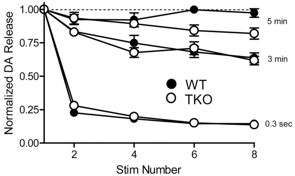
Figure 3. The effects of repetitive stimuli on DA release. Single stimuli were applied at intervals of 0.3 sec, 3 min, and 5 min, and the amount of DA released in response to each stimulus was normalized to the amount of DA released in response to the first stimulus.
