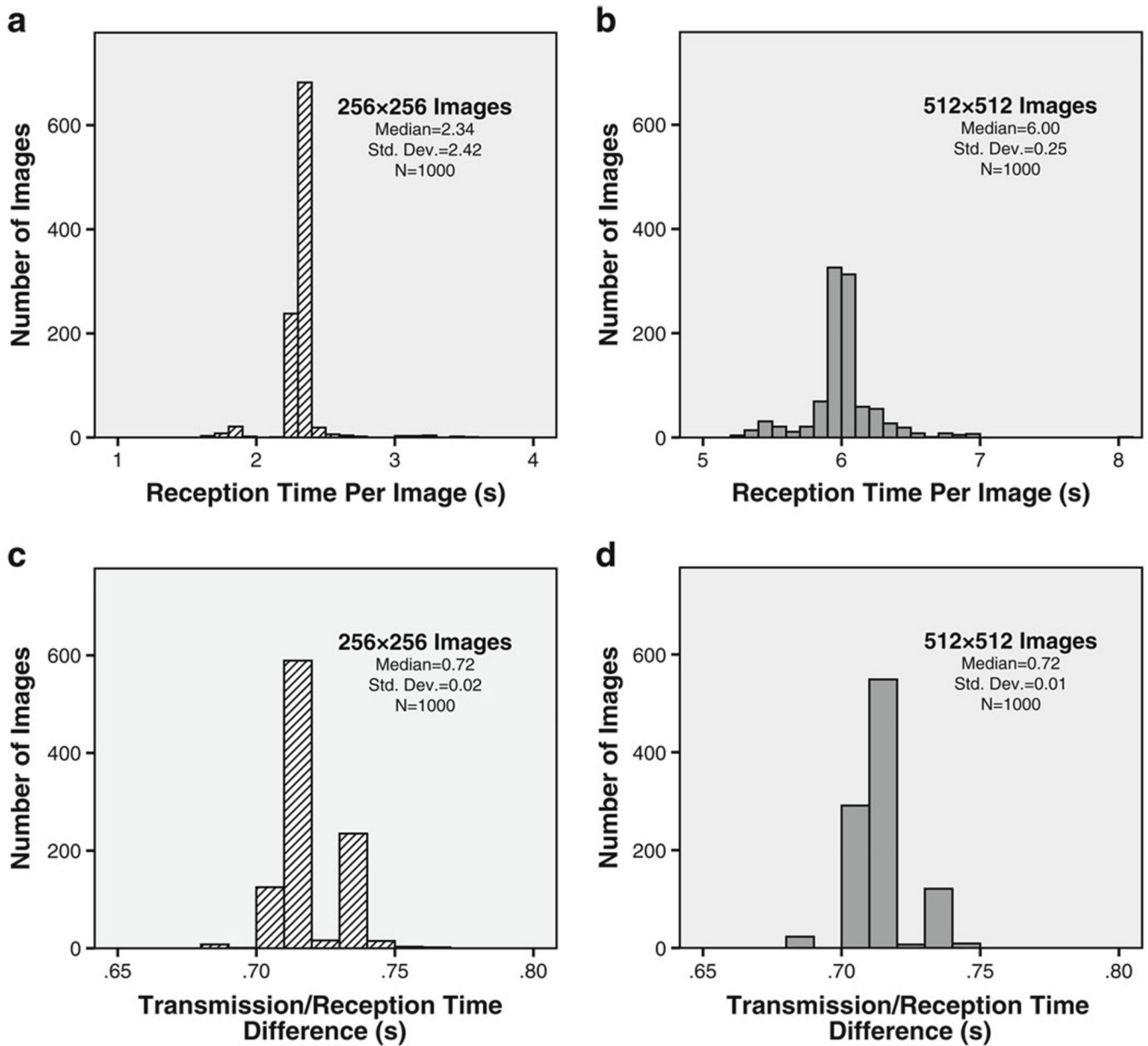
Fig. 4. Image transit time histograms for transmitting a synthetic study comprising 1,000 duplicate MR images that were 256x256 for (a) and 512x512 for (b). c, d The respective differences in transmission time as measured by the sending and receiving DICOM routers. The c and d difference histograms are effectively showing the distribution of round-trip network latency and hence are very similar.
