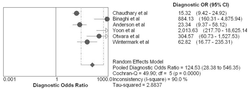
Fig 2. Forest plot of the DOR for the CTA meta-analysis. The DOR for each research study is represented by circles. The 95% CI is represented by the horizontal lines through each circle. The pooled DOR for this meta-analysis is represented by the diamond symbol.
