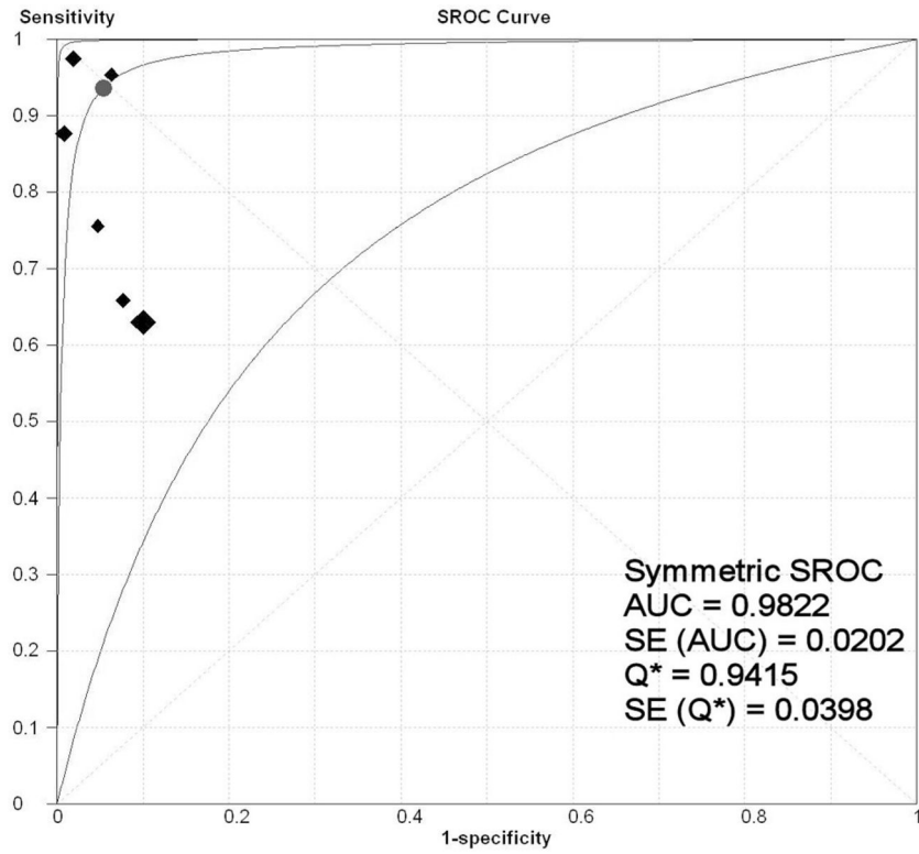
Fig 1. SROC curve for the CTA meta-analysis. Each black diamond represents an individual research study in the CTA meta-analysis, with the size of the diamond directly proportional to the sample size of the study. The best fit curve (middle curve) lies between the other 2 curves, which demarcate its 95% CI. The circle denotes the Q*-point.
