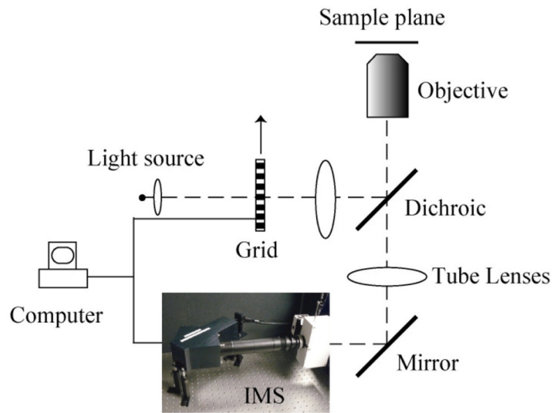
Fig. 1. Depth-resolved IMS with SI.
