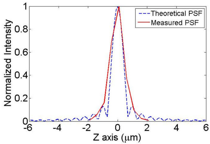
Fig. 2. Axial PSF measurement in the depth-resolved IMS.
