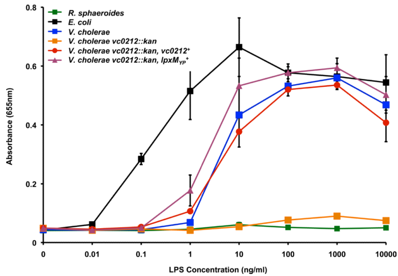
Figure 8. LPS from vc0212 deletion mutant does not stimulate innate immune recognition by human TLR4-MD2
