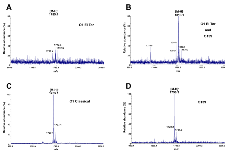
Figure 2. MALDI-TOF mass spectrometry of V. cholerae serogroups O1 and O139
