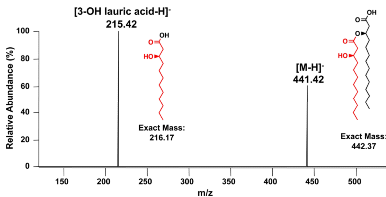
Figure 6. MS 3 spectrum of lipid A isolated from E. coli MLK1067 expressing Vc0212 The doubly deprotonated lipid A ion (m/z 891.5) from MLK1067 expressing Vc0212 was subjected to 193 nm UVPD (see Figure S4) followed by CID of the fragment ion of m/z 441.4. The ion of m/z 441.4 is interpreted as the deprotonated intact 3'-acyloxyacyl moiety of lipid A (exact mass calculated to be 442.37 u, proposed structure shown in the spectrum). The MS 3 fragment ion of m/z 215.42 is interpreted as deprotonated 3-hydroxy lauric acid (exact mass 216.17 u, proposed structure shown in the spectrum).
