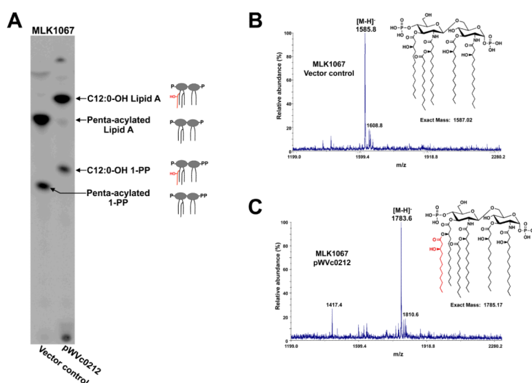
Figure 5. Heterologous expression of Vc0212 in the E. coli lpxM deficient strain MLK1067 ^{32}\text{P} -labeled lipid A species from MLK1067 expressing pWSK29 and pWVc0212 were analyzed by TLC and visualized by phosphorimaging (panel A). Major lipid A species are indicated with arrows. Lipid A species of MLK1067 containing pWSK29 (panel B) and pWVc0212 (panel C) were analyzed by MALDI-TOF mass spectrometry. The major peak in panel B is m/z 1585.8, which corresponds to the expected mass of deprotonated penta-acylated lipid A. The major peak in panel C is m/z 1783.6, indicative of the addition of a 3-hydroxylaurate (3-OH C12:0) to the glucosamine disaccharide of the lipid A species. Minor peaks at m/z 1608.8 and m/z 1810.6 are likely sodium adducts of the lipid A species. The predicted structure of the major lipid A species for each strain is shown.
