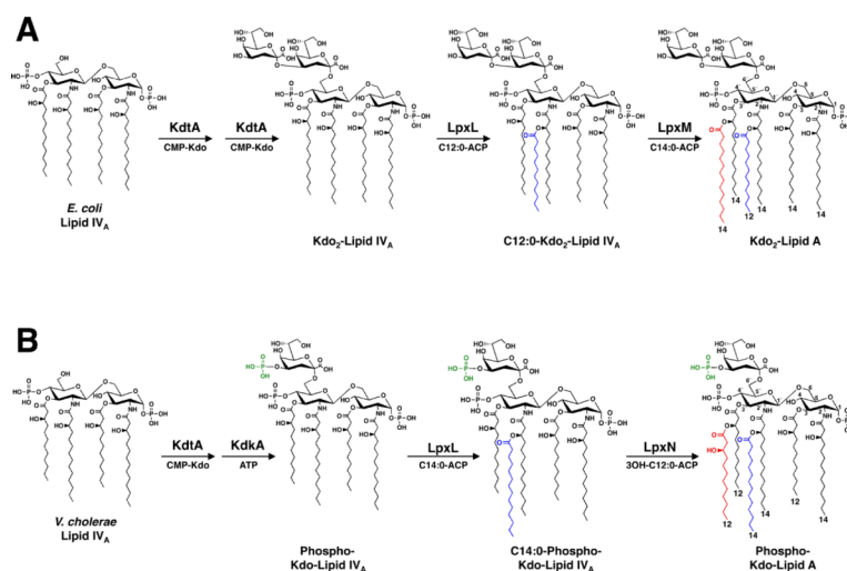
Figure 1. Comparison of the late stages of Kdo-lipid A biosynthesis in E. coli and V. cholerae (A) E. coli possess a bifunctional Kdo transferase (KdtA, also known as WaaA), which transfers two Kdo sugars to the lipid A precursor lipid IV A . The lipid A secondary acyltransferases, LpxL and LpxM then catalyze the transfer of a laurate (C12:0) (blue) to the 2'-position and a myristate (C14:0) (red) to the 3'-position of the glucosamine disaccharide, creating Kdo 2 -lipid A. (B) The V. cholerae genome encodes a monofunctional KdtA, which transfers one Kdo residue to lipid IV A . The Kdo kinase (KdkA) then phosphorylates the Kdo sugar (green), resulting in phosphorylated Kdo-lipid IV A . V. cholerae LpxL (Vc0213) catalyzes the transfer of a myristate (C14:0) (blue) to the 2'-position of the glucosamine disaccharide. As shown in the current work, LpxN (Vc0212) transfers a 3-hydroxylaurate (3-OH C12:0) (red) to the 3'-position, generating the hexa-acylated V. cholerae Kdo-lipid A domain. The exact order in which the secondary acyl chains are added in V. cholerae has not been determined.
