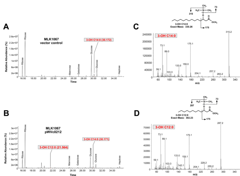
Figure 7. GC/MS analysis of hydroxylated fatty acids from LPS isolated from E. coli MLK1067 expressing Vc0212
