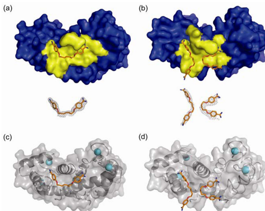
Figure 3. High-resolution crystal structures of S100B bound to heptamidine and pentamidine. (a) and (b) Surface representation of the structure of S100B bound to heptamidine (a) and pentamidine (b). Residues within 3 Å are colored yellow to highlight the binding pocket. Below, the electron density maps calculated with the 2mF_o-DF_c coefficients (contoured at 1.0\sigma ) for each compound are shown. The atoms of the compound are colored orange (carbon), blue (nitrogen), and red (oxygen). (c) and (d) Cartoon representation of the structure of S100B bound to heptamidine (c) and pentamidine (d) with helices visible. Compounds are colored as in (a) and (b) and calcium ions are depicted as cyan spheres.
