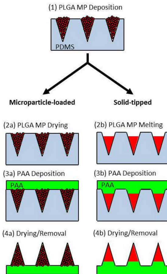
Figure 1. Schematic view of composite microparticle and bulk PLGA tip microneedle array fabrication. PDMS molds were first filled with PLGA microparticles through centrifugation (1). PLGA microparticles were then either dried in mold cavities (2a) or fused at high temperature to create a solid tip (2b). Concentrated aq. PAA solution was then centrifuged onto the filled molds to create a supportive matrix (3a) or pedestal (3b) for rapid dissolution in vivo . After drying microneedles were removed from PDMS molds (4a, 4b).
