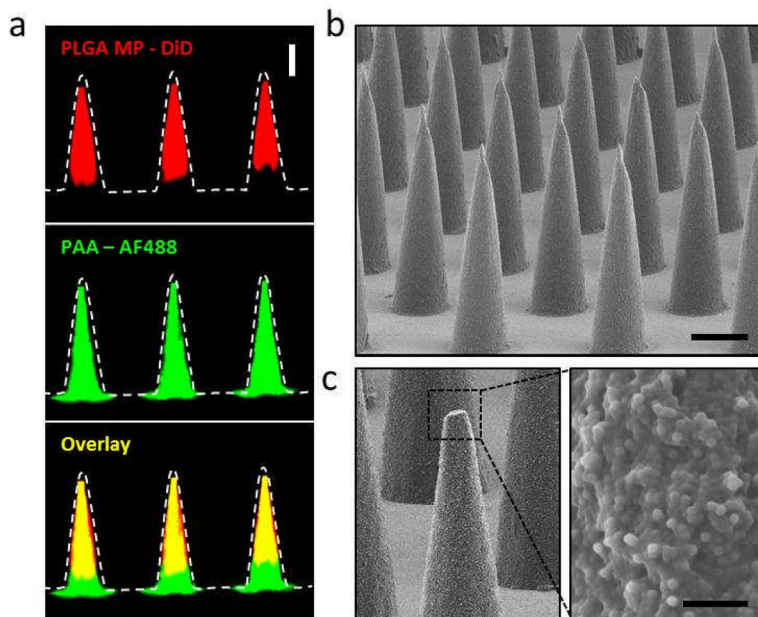
Figure 2. a) Confocal micrographs of PLGA-PAA composite microneedles fabricated to encapsulate DiD-loaded PLGA microparticles (MP) (right, scale bar 200 \mu\text{m} ). SEM micrographs of b) resulting microparticle-encapsulating microneedle array (scale bar 200 \mu\text{m} ) and c) high magnification image of the composite needle interior of a fractured microneedle (scale bar 10 \mu\text{m} ).
