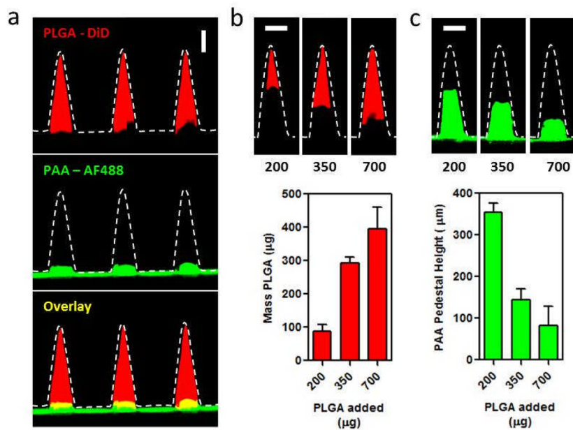
Figure 3. a) Confocal micrographs of PLGA-PAA composite microneedles fabricated with a PAA base and DiD-loaded solid PLGA tip (scale bar 200 µm). Confocal micrographs of microneedles fabricated with varying amounts of DiD-loaded PLGA microparticles as indicated giving a range of PLGA tip sizes (b) and PAA pedestal heights (c).
