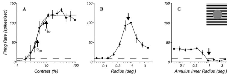
Fig 1. Contrast-response and size tuning for a complex cell. A: the response as a function of contrast for a grating of the optimal orientation, spatial and temporal frequency and drift direction, presented in a circular window that was the optimal size for the classical receptive field (CRF). The solid line is the best-fitting Naka-Rushton function. The arrows show the contrast eliciting 50% ( C_{50} ) and 90% ( C_{90} ) of the maximum response of the neuron, which were the contrasts used for subsequent contextual experiments. The dashed line indicates the spontaneous firing rate. B: the response as a function of the radius of the circular window containing an optimal grating as described above in (A). The arrow shows the smallest window radius eliciting the peak response of the neuron, which is the size of the central patch used in subsequent contextual experiments. C: a full field optimal grating was presented that included a central grey circular region, where the radius of the central region varied from 0 to 4 degrees, in 1/2 octave steps. The arrow shows the smallest radius of central blank grey region that elicited no response from the neuron. This size was used as the inner radius of stimuli presented to the extra-classical receptive field (eCRF) and the outer radius of the grey annulus separating stimuli in the CRF from the eCRF (see the configuration in Fig. 2B, C).
