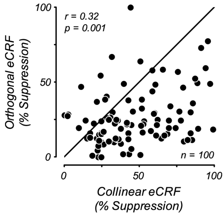
Fig. 5. Orientation-dependent eCRF suppression strength. Scatter plot of the maximum strength of suppression from collinear and orthogonal stimuli in the eCRF. Suppression strength was defined as the percent suppression of CRF responses and was estimated as the R_{max} parameter from contrast-response function fits to eCRF suppression. There was a significant correlation between the strength of eCRF suppression for collinear and orthogonal stimuli ( r = 0.32 , p = 0.001 ). Nearly all points lie below the unity line, indicating that there was consistently stronger suppression from the collinear eCRF stimulus.
