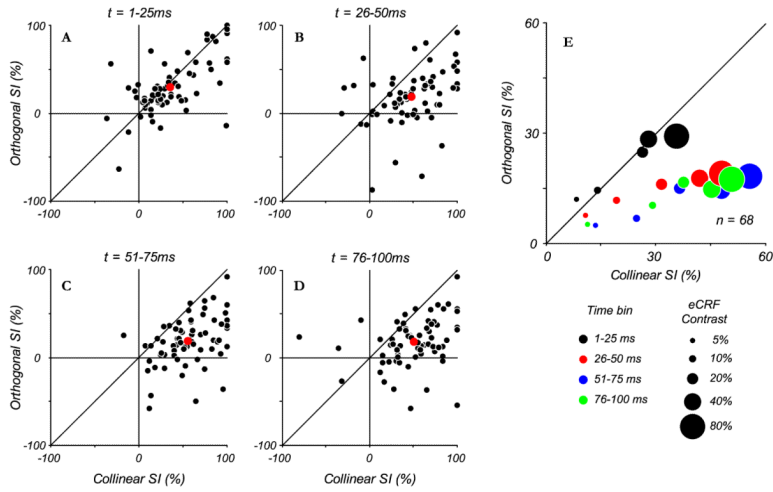
Fig. 11. Comparison of suppression to collinear and orthogonal stimuli over time. Suppression indices for 68 complex cells for collinear and orthogonal eCRF stimuli at 80% contrast were calculated as a function of time in 25 ms bins, where t is time from CRF response onset, and 100% represents complete suppression of the response and 0% represents no suppression, negative SI values indicate response facilitation. A: at the earliest times (1-25 ms) the amount of suppression was approximately equal between the two conditions, as shown by points lying along the unity line. The point in red indicates the mean suppression over all neurons. B: at later times (26-50 ms), stronger suppression from the collinear eCRF stimulus started to become evident, which persisted at later time points (C, D). E: the average suppression indices are plotted for the population of cells to illustrate how suppression developed across time and across contrasts. The size of the dot indicates the contrast presented in the eCRF, with larger sizes indicating higher contrasts. The color of the dot indicates the time bin over which the suppression indices were measured. At earliest times (black) the suppression between the two stimuli was equal, with higher contrasts inducing greater suppression. At later time points (red, blue, green), for all contrasts, suppression from the collinear stimuli in the eCRF was greater than from orthogonal stimuli.
