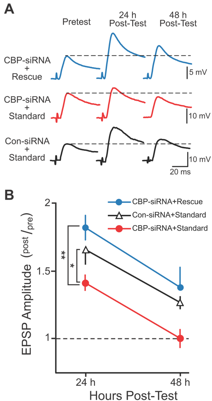
Figure 4. Rescue Protocol compensated for the CBP knockdown
