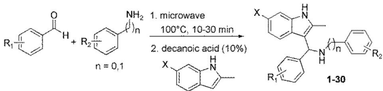
Scheme 1. Improved synthesis of 3-indolylmethanamines
