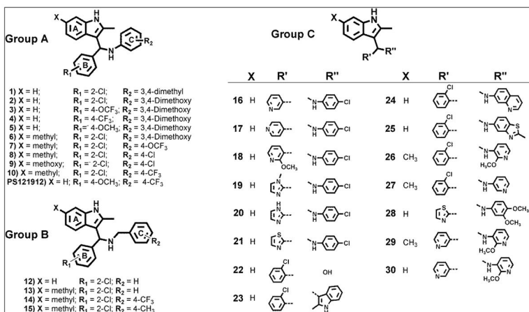
Figure 1. Structures of synthesized 3-indolylmethanamines.
