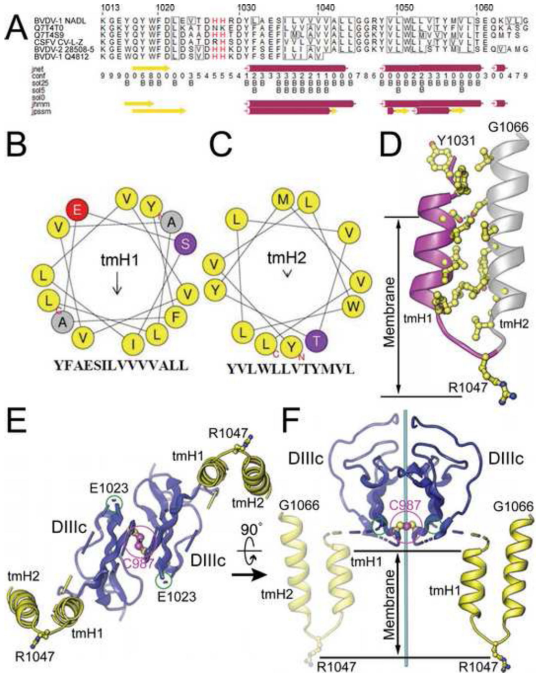
Figure 2. Sequence analysis and atomic modeling of the BVDV E2 membrane anchor. (A) Two transmembrane helices (tmH1 and tmH2) were predicted with JPRED-3. The reference sequence and numbering refer to the BVDV-1 NADL polyprotein (Xu et al., 1997). This sequence was used to query the UniRef90 database. The following pestivirus E1 UniProt sequences returned from the search are shown: Q7T4T0, Pestivirus PG-1; Q7T4S9, border disease virus strain V2536/2; Q9WPE6, classical swine fever virus strain C-V-LZ; Q9WP29, BVDV-2 strain 28508-5; Q65793, BVDV-1 strain Q4812. (B–C) Helical wheel
