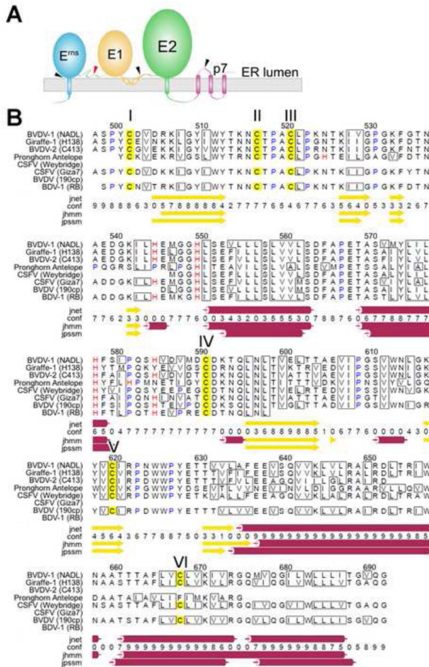
Figure 3. Topology and secondary structure predictions of BVDV E1. (A) Topology of the pestivirus E1 and E2 proteins. Wedges indicate the sites at which proteases cleave during polyprotein maturation. (B) Secondary structure prediction of BVDV E1 based on a pestivirus multiple sequence alignment. Secondary structure elements were predicted with Jpred 3. Sequence numbering refers to the BVDV-1 NADL polyprotein. The sequence contains six cysteines, labeled I–VI and referred to in the text as such. Conserved His residues flank the first two predicted \alpha -helices. The following pestivirus E2 UniProt sequences were selected for the
