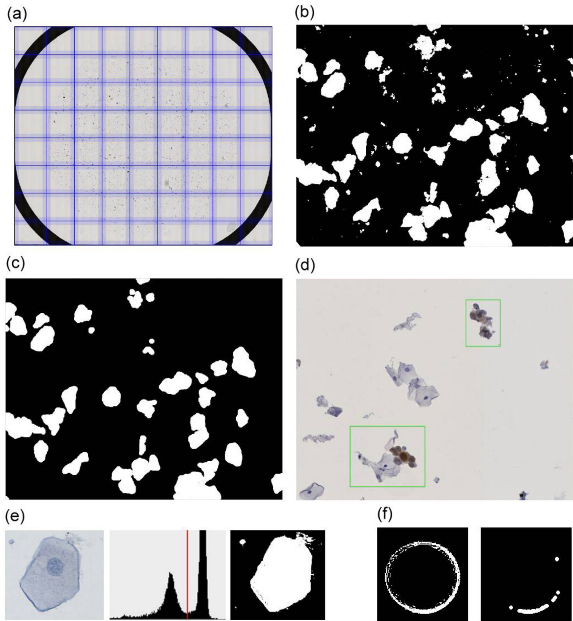
Figure 2. Illustration of object detection
