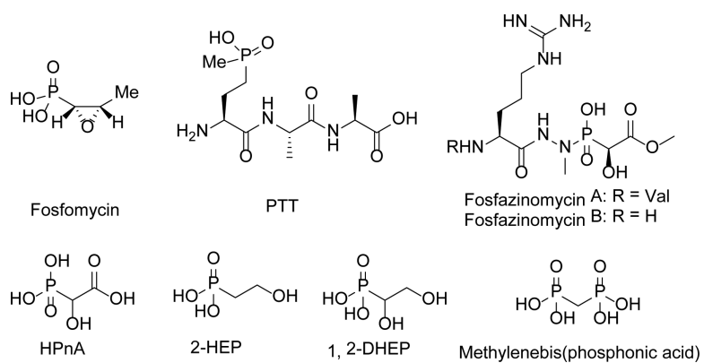
Figure 1. Structures of select phosphonates.
