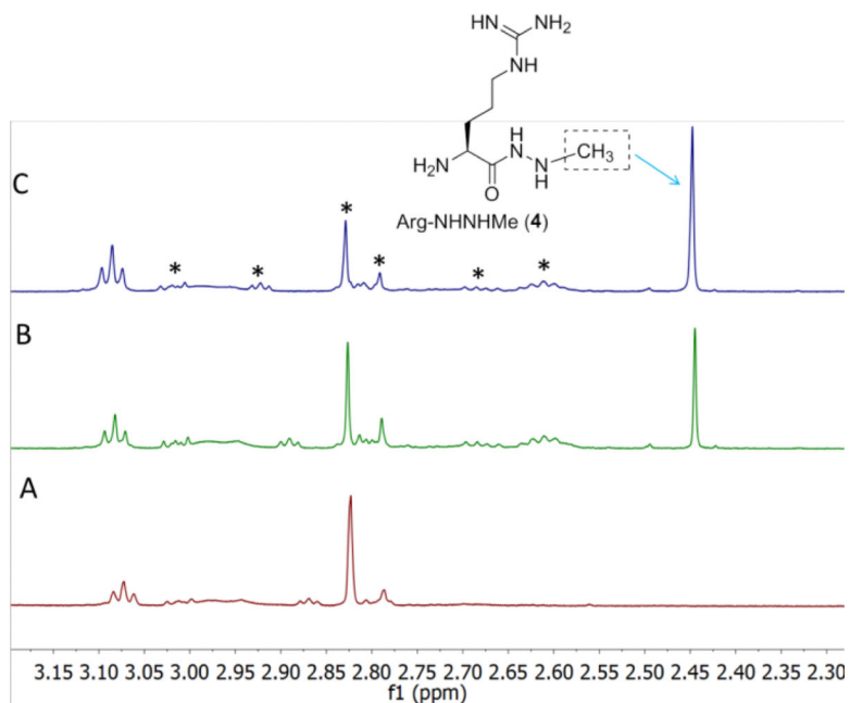
Figure 5. ^1\text{H} NMR spectra of products generated upon incubation of His 6 -FzmH with Arg-NHNH 2 (3). A. NMR spectrum of the reaction mixture in the absence of His 6 -FzmH. B. NMR spectrum of the enzymatic reaction mixture containing Arg-NHNH 2 , SAM, AdoHcy nucleosidase, and His 6 -FzmH. C. NMR spectrum of the reaction mixture spiked with authentic standard of Arg-NHNHMe. The peaks marked with asterisks originate from SAM and SAM-related products.
