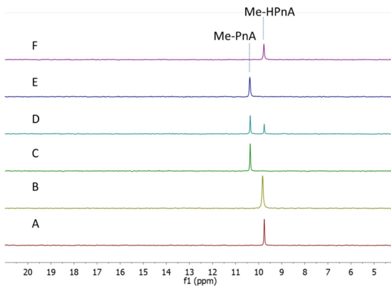
Figure 3. ^{31}\text{P} NMR spectra of the products obtained by incubation of His 6 -FzmG with Me-PnA. A. NMR spectrum of the reaction mixture containing Me-PnA, O 2 , \alpha -KG, Fe(II), L-ascorbate, and His 6 -FzmG. B. NMR spectrum of the enzymatic reaction mixture spiked with authentic standard of Me-HPnA. C. NMR spectrum of the reaction mixture in the absence of \alpha -KG. D. NMR spectrum of the reaction mixture in the absence of L-ascorbate. E. NMR spectrum of the reaction mixture in the absence of His 6 -FzmG. F. NMR spectrum of authentic Me-HPnA.
