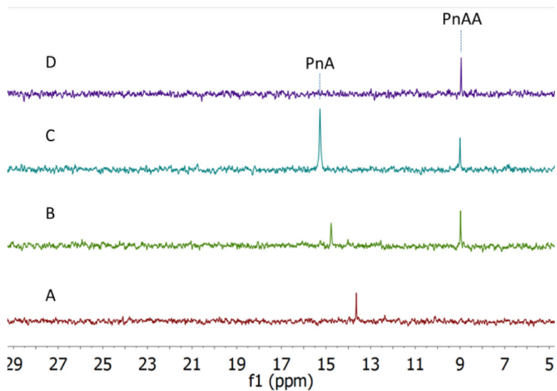
Figure 4. ^{31}\text{P} NMR spectra analysis of the incubation of His 6 -FzmG with PnAA. A. NMR spectrum of the reaction mixture containing PnAA, O 2 , \alpha -KG, Fe(II), L-ascorbate, and His 6 -FzmG. B. NMR spectrum of the enzymatic reaction mixture spiked with authentic standard of PnAA. C. NMR spectrum of the reaction mixture spiked with authentic standards of PnAA and PnA. D. NMR spectrum of the reaction mixture in the absence of His 6 -FzmG. The chemical shifts of phosphonates in ^{31}\text{P} NMR are very sensitive to pH near their \text{p}K_{\text{a}} values, accounting for the changes in chemical shifts between experiments and requiring spiking with standards for assignments.
