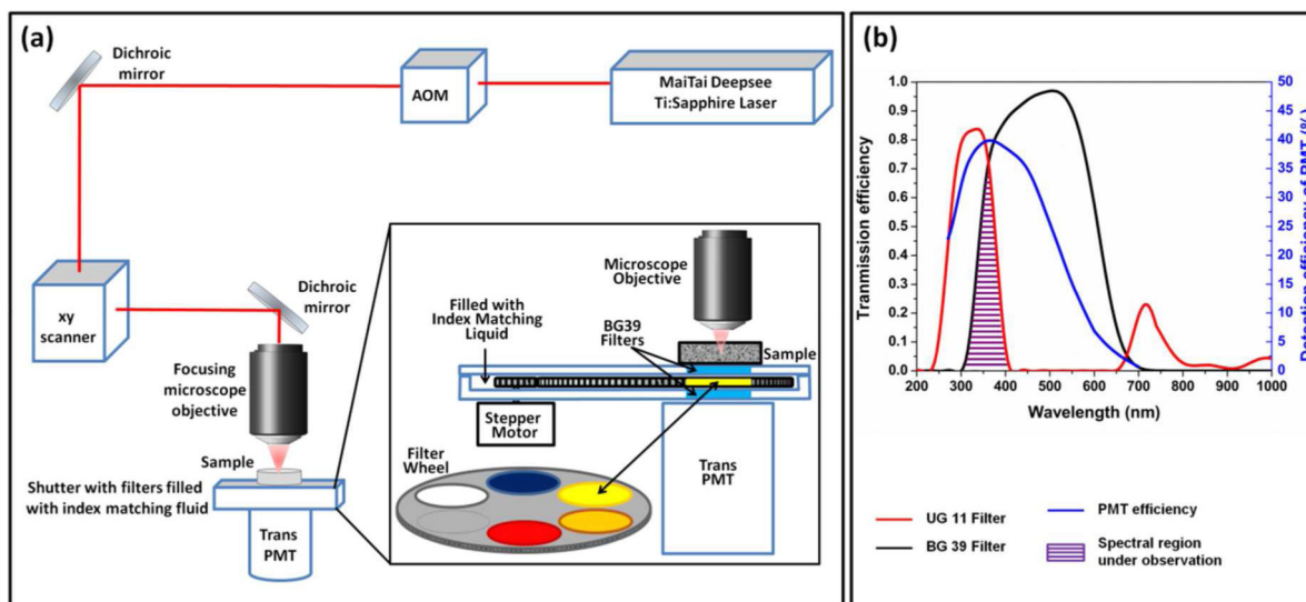
Figure 1. Schematic representation of the DIVER microscope set up. 25,26 (a) The upright excitation scheme and positioning of sample directly on top of wide area PMT. The inset shows the construction of the filter wheel assembly. (b) Overlap of the transmission spectra of the filters used, UG11 (red line) and BG39 (black line), and the detection efficiency of the PMT (blue line). The overlapped wavelength area (purple) is used for detection of tryptophan fluorescence.
