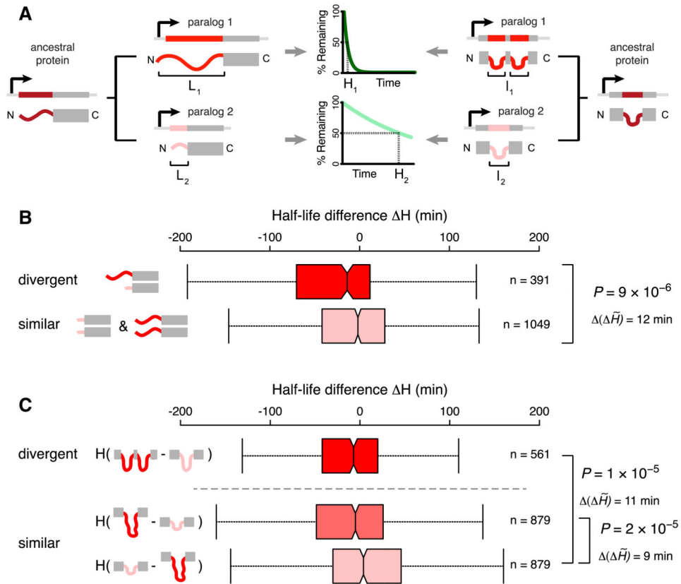
Figure 4. Divergence in Disordered Segments during Evolution Can Impact Protein Half-Life (A) Schematic depiction of how the half-life of paralogs could be altered by changes in N-terminal and/or internal disordered segments during evolution. The dark and light green degradation curves denote a short and long half-life. This schematic is not intended to cover all possible scenarios for divergence of disordered segments between paralogs. (B) Distributions of half-life differences ( \Delta H ) in pairs of yeast paralogs, grouped according to the difference in the length of their N-terminal disordered segments. Top: one paralog has a short and the other paralog a long disordered N terminus (SL). Bottom: both paralogs have short (both \leq 30 residues; SS) or both have long (both >30 residues; LL) disordered N termini. (C) Distribution of half-life differences ( \Delta H ) in paralog pairs, grouped according to the difference in the number of internal disordered regions ( \Delta I ). Top: pairs where one of the two paralogs has a higher number of internal disordered segments ( \Delta I = 1 ). Bottom: pairs with identical numbers of internal disordered segment ( \Delta I = 0 ). Each paralog pair is arranged so that \Delta L = L_1 - L_2 (B) and \Delta I = I_1 - I_2 (C) are always positive (i.e., L_1 \geq L_2 and I_1 \geq I_2 ). This order is used for the \Delta H calculation (that is, the half-life of the paralog with the shortest N-terminal disorder, or the smallest number of internal disordered segments, will be subtracted from the half-life of the other one; \Delta H = H_1 - H_2 ). As a result, \Delta H will be negative for pairs where an increase in N-terminal or internal disorder coincides with a shorter half-life (Experimental Procedures). For \Delta I = 0 (C, bottom), two \Delta H distributions were obtained by ordering the paralogs within a pair according to the total length of all internal disordered segments (increasing and decreasing
