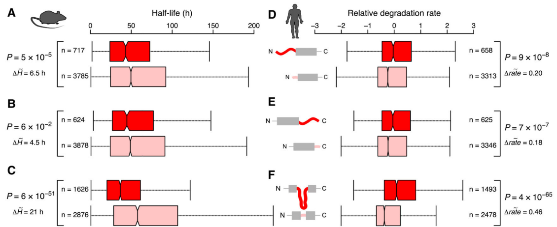
Figure 3. The Effects of Disordered Segments on Protein Turnover in Mouse and Human Boxplots of the distributions of half-life values in Mus musculus (A–C), and relative degradation rates in Homo sapiens (D–F), for proteins with long and short N-terminal, C-terminal, and internal disordered segments. Note that the scale for protein half-life is in hours for mouse, rather than minutes as in yeast. Values are reversed for the human data: proteins with a short half-life have a high relative degradation rate. See Figure 1 for further information. See also Table S5.
