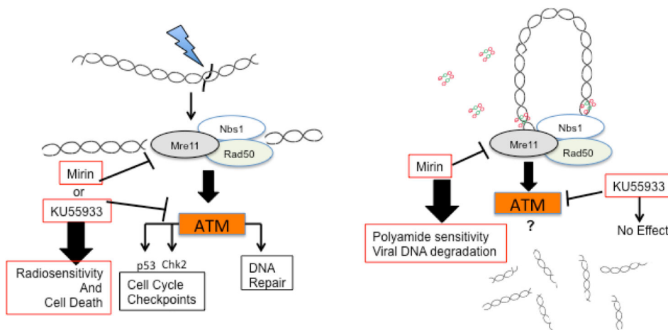
Figure 4. Mirin is an antiviral polyamide (AVP) sensitizer. Inhibition of MRE11 promotes the effectiveness of chemo- and radio-therapy (left) and antiviral polyamides (AVPs) (right). Inhibitors of DNA repair processes increase cell sensitivity toward therapeutic irradiation and chemotherapeutic agents that act by damaging cellular DNA. Inhibition of, for example, MRE11 or ataxia-telangiectasia mutated (ATM) augments cell death in response to DNA damage by preventing cell cycle arrest and DNA repair. In an analogous manner, Mirin (but not ATM inhibitor KU55933) promotes the degradation of HPV episomal DNA in response to AVPs. MRE11 therefore has a role that protects viral episomes from AVPs that does not require signaling through the ATM/CHK2 pathway [6].
