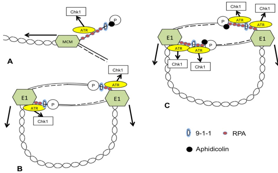
Figure 5. Putative model for instability of HPV episomes in presence of ATR/CHK1 inhibitors or aphidicolin. Simplified models of vertebrate replication fork in presence of aphidicolin (A) and HPV replication fork in the absence (B) or presence (C) of aphidicolin are shown. (A) Aphidicolin inhibition of polymerase in vertebrate cells results in continued activity of the MCM helicase, exposure of ssDNA, and activation of the ATR/CHK1 pathway to stabilize the fork; (B) E1 activity reportedly activates ATR and ATM, and inhibition of ATR/CHK1 results in loss of episomes suggesting that that ATR normally stabilizes viral replication fork; (C) It's proposed that polymerase inhibition by aphidicolin along with continued E1 helicase activity results in additional exposure of ssDNA, activation of ATR/CHK1 pathway, and accumulation of unstable replication intermediates which are degraded by the cell.
