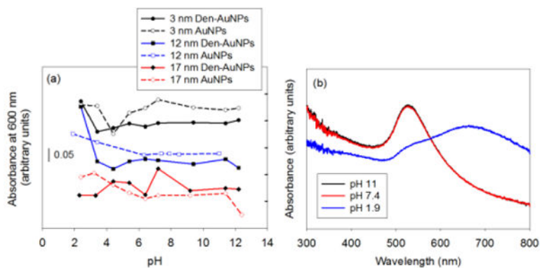
Fig. 6. The pH stability results of AuNPs and Den-AuNPs with different core sizes: (a) absorbance at 600 nm at different pH and (b) UV-vis spectra of 12 nm AuNPs at selected pHs are displayed to show the increase in absorbance at 600 nm and the red-shifts of SP bands resulting from aggregations.
