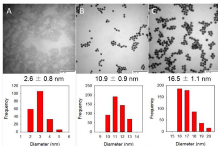
Fig. 4. TEM images and histograms of Den-AuNPs: (a) 2.6 \pm 0.8 nm, (b) 10.9 \pm 0.9 nm and (c) 16.5 \pm 1.1 nm. The scale bars in all three TEM images are 100 nm.
