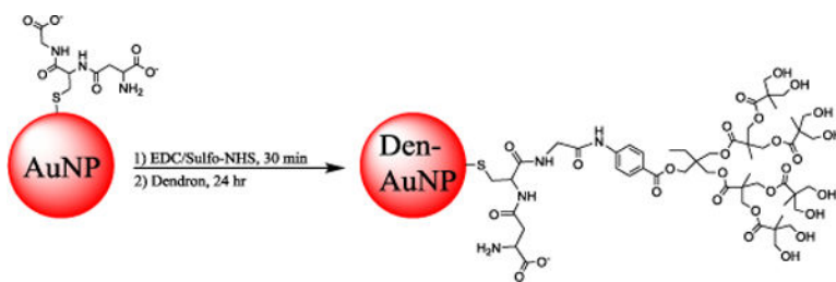
Scheme 1. Synthesis of dendron-conjugated gold nanoparticles (Den-AuNPs).
