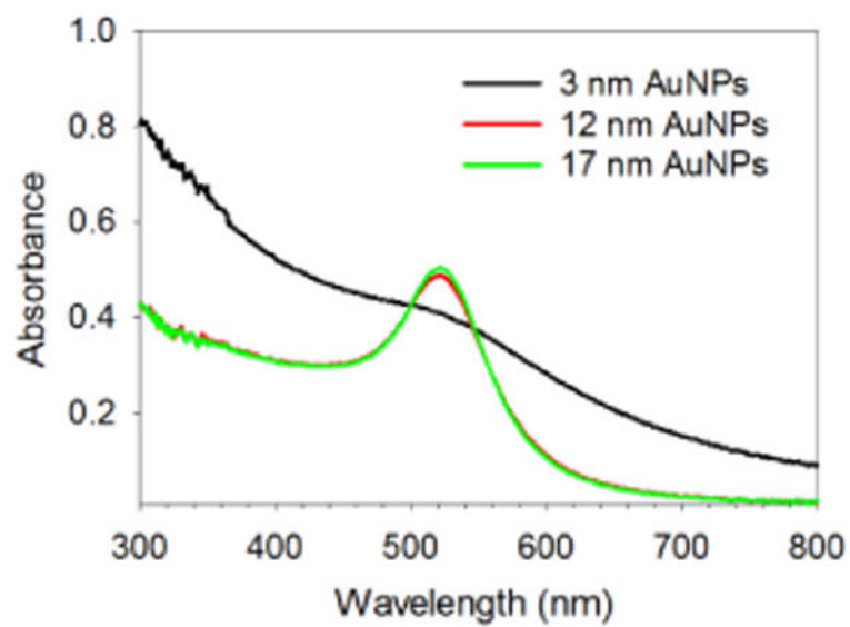
Fig. 2. UV-vis spectra of 3, 12 and 17 nm AuNPs dissolved in PBS buffer solution. The concentration of AuNPs is \sim 0.1 mg/mL.
