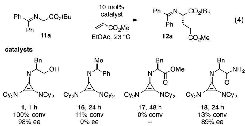
Figure 3. Necessity of H-bonding functionality for high reactivity and enantioselectivity.
