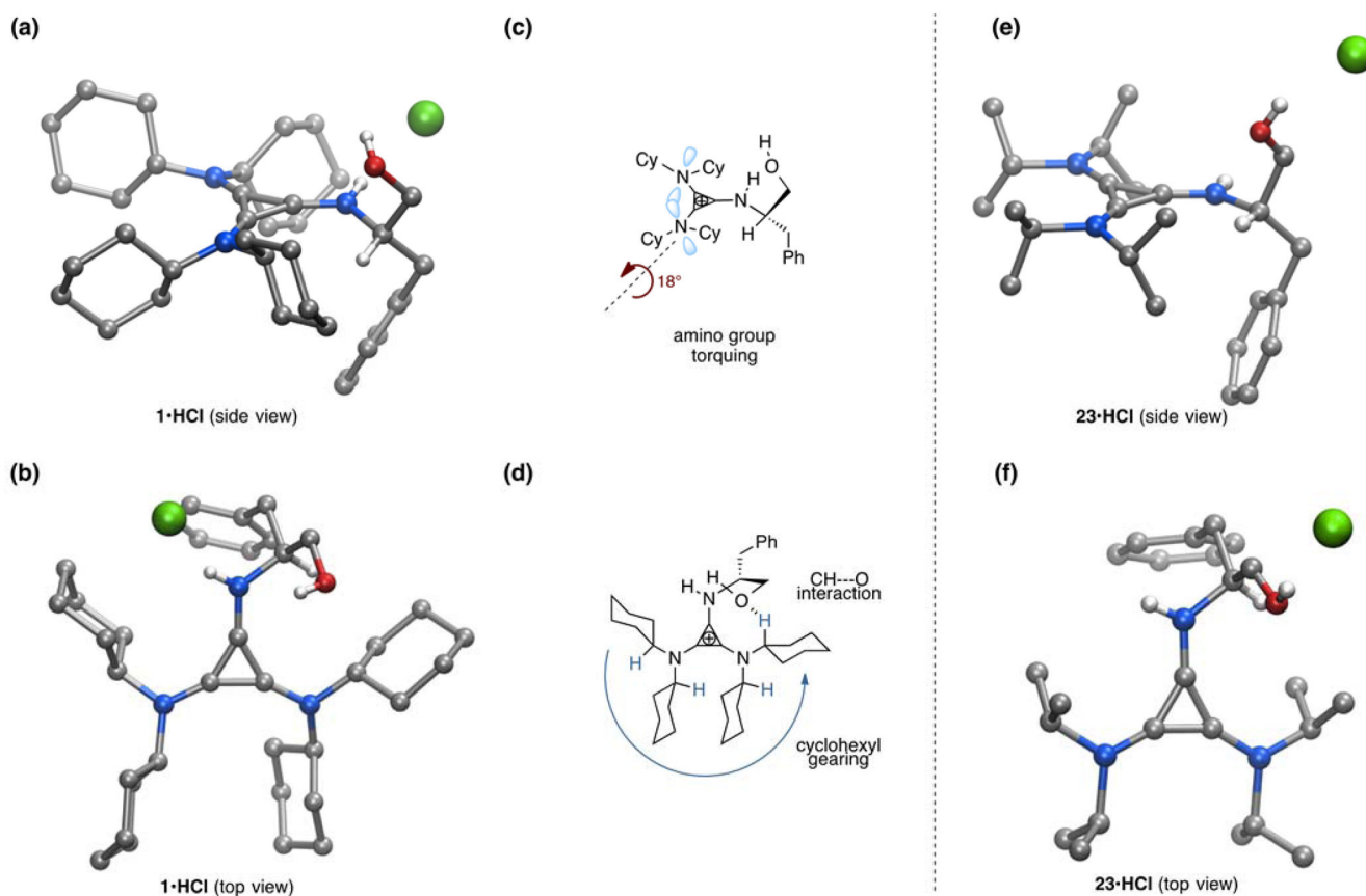
Figure 4. Molecular structure of (a) 1 •HCl side view; (b) 1 •HCl top view; (c) Depiction of amino group torquing phenomenon of 1 •HCl; (d) Depiction of cyclohexyl gearing effect and key CH...O interaction of 1 •HCl; (e) 23 •HCl side view; and (f) 23 •HCl top view. For (a) and (b) a co-crystallized molecule of H 2 O has been omitted for clarity. For (e) and (f) the hydroxymethyl group was disordered and only one of the crystal forms is shown for clarity. A molecule of co-crystallized benzene was also removed for 23 -HCl. The unmodified structures are included in the supporting information file.
