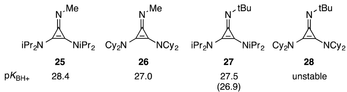
Figure 5. Basicities of representative cyclopropenimines. The pK_{BH^+} values were determined by ^1H NMR in d_3 -MeCN in reference to the P_1 -tBu phosphazene base. The number in parentheses is the value previously determined by an alternative method.
