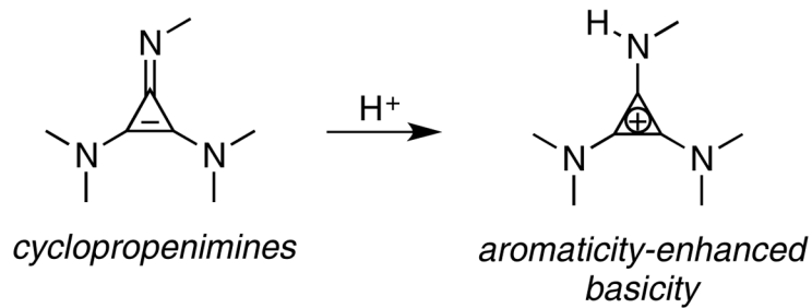
Figure 1. Enantioselective Brønsted base catalysis with cyclopropenimine 1 .
