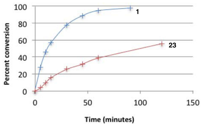
Chart 1. Conversion rates of catalysts 1 and 23 .
