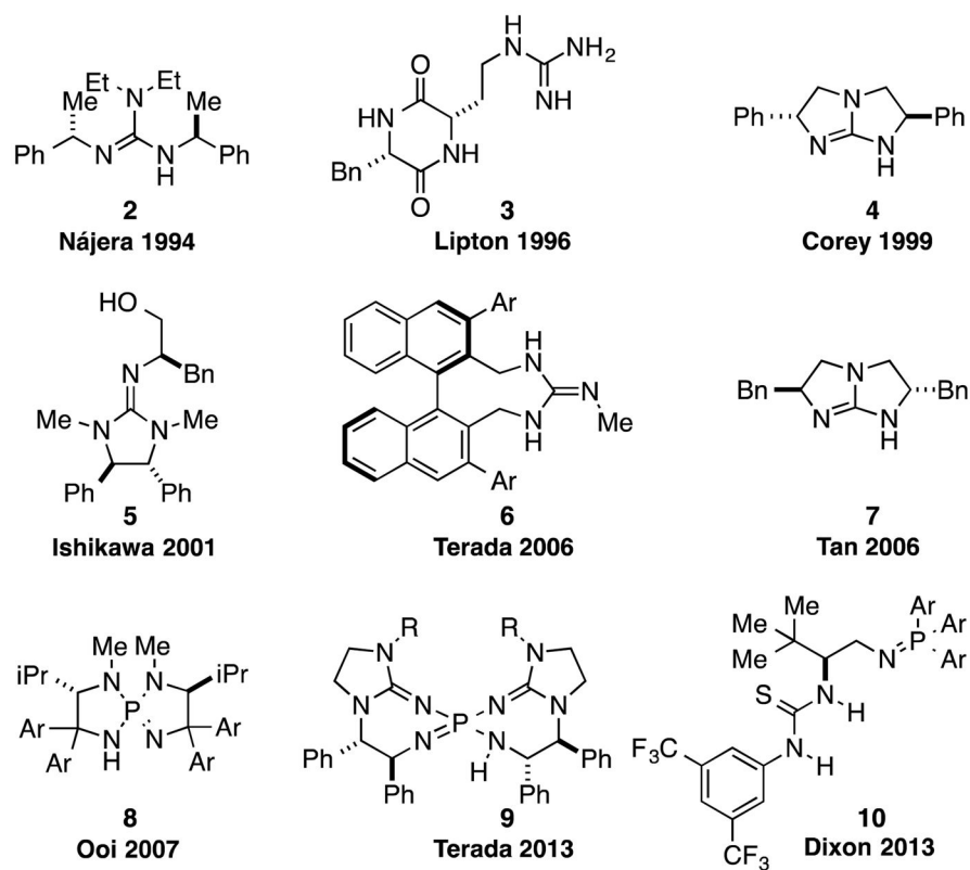
Figure 2. Examples of chiral Brønsted base catalysts with strong basicities.
