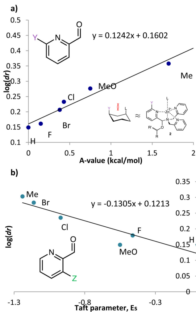
Figure 3. Linear plots showing \log(dr) values for assemblies involving a) 6-substituted pyridine-2-carbaldehydes plotted against A-values corresponding to the substituents, and b) 3-substituted pyridine-2-carbaldehydes plotted against corresponding Taft steric parameters.
