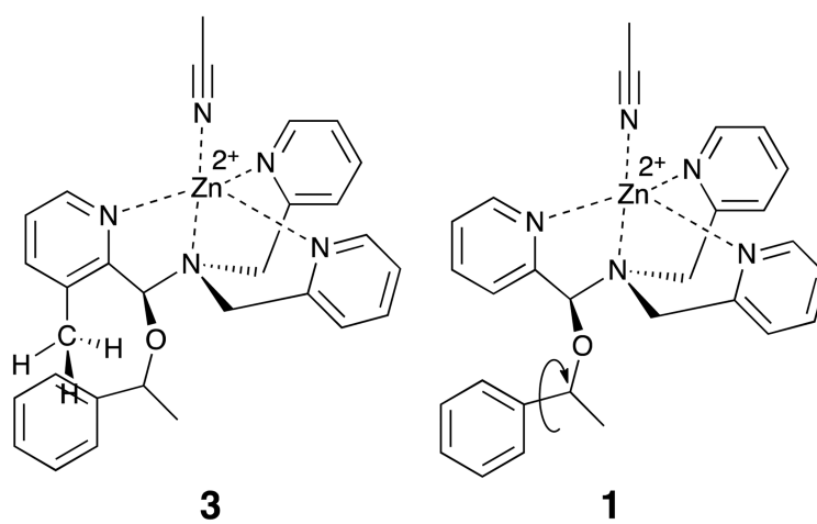
Figure 8. Proposed origin of context dependent steric size. Assembly 3 , with an additional proximal methyl group, hinders the alcohol phenyl substituent rotation.
