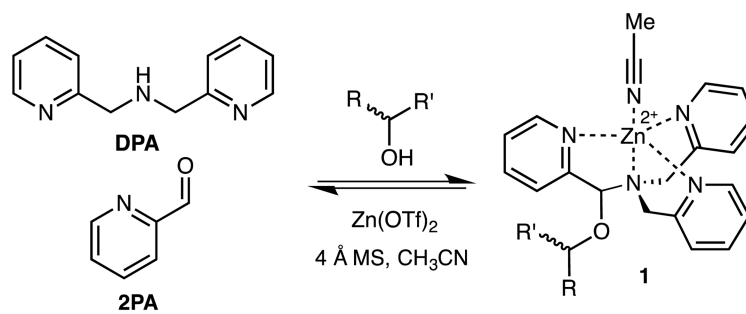
Figure 1. Multicomponent hemiaminal ether assembly ( 1 ), formation from 2-pyridinecarbaldehyde ( 2PA ), di(picoly)amine ( DPA ), Zn 2+ , molecular sieves (3Å), and a chiral alcohol analyte.
