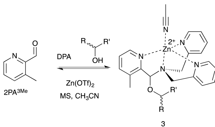
Figure 4. Multicomponent assembly 3 formed with ligand 2PA 3Me , DPA , Zn(OTf) 2 , and chiral alcohol following the same protocol as reported above.
