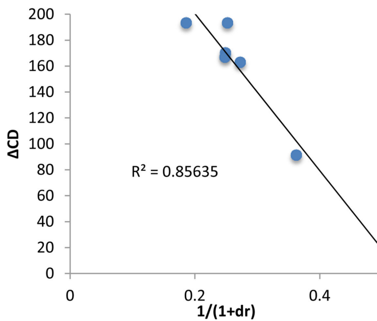
Figure 6. The alcohol dr value was correlated to their enantiopure sample CD value at 270 nm using assembly 3 .
