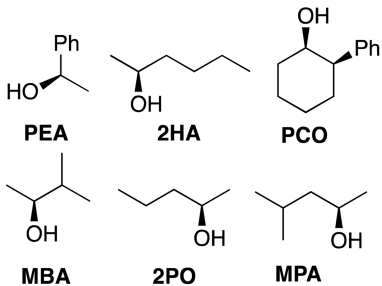
Figure 5. The alcohols used in the correlating alcohol steric size to their corresponding CD signal
