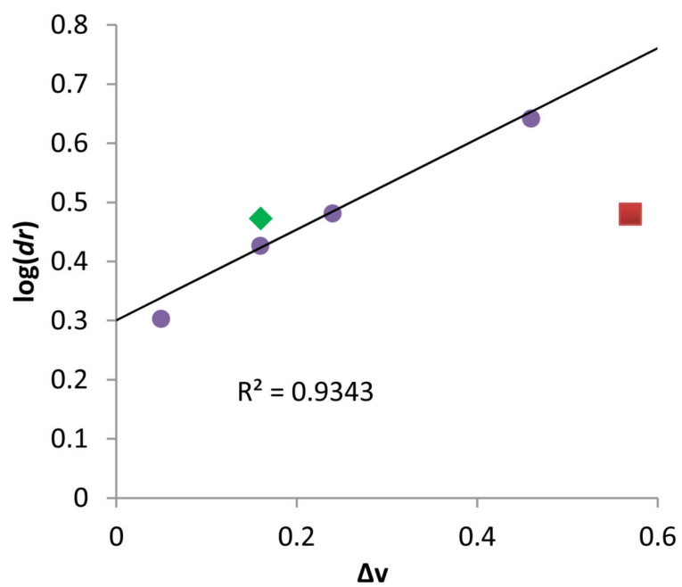
Figure 7. Linear correlation was established between the alcohol substituent Charton parameters ( \nu ) and their corresponding \log(dr) value.
