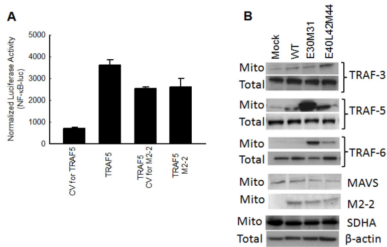
Figure 3. PDZ Motifs 29-DEMI-32 and 39-KEALSDGI-46 of M2-2 protein suppress IRF-3 and NF-κB activation by inhibiting mitochondrial signalosome formation
