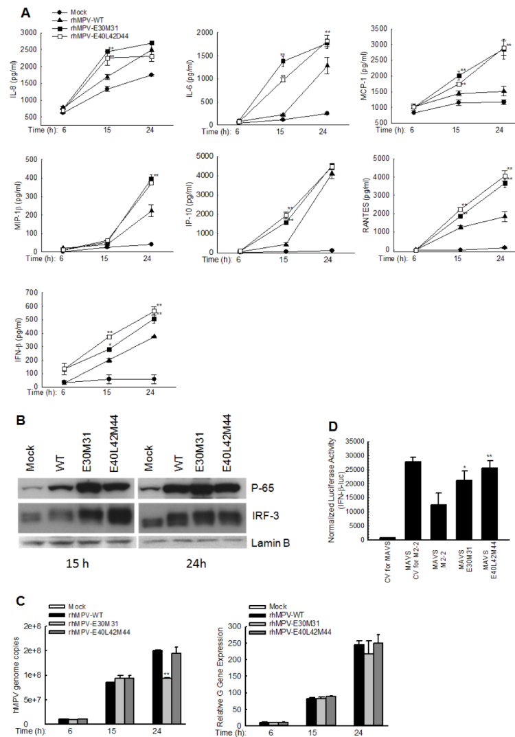
Figure 1. PDZ Motifs 29-DEMI-32 and 39-KEALSDGI-46 are important for hMPV-induced innate immune responses
