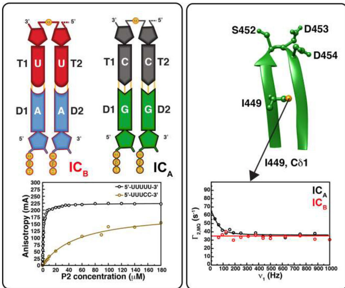
Figure 8. Slow timescale dynamics in P2
