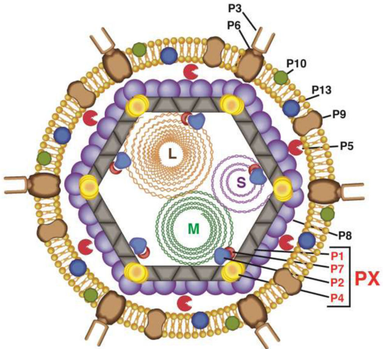
Figure 1. Schematic representation of the structural organization of a mature cystovirus virion The membrane proteins that include the major envelope protein, P9 (90 residues in \Phi 6 ), an envelope protein, P10 (42 residues), and a minor membrane protein, P13 (72 residues) are associated with the outer lipid envelope. Exposed to the extracellular medium, is the receptor-binding spike protein, P3 (648 residues) that forms a complex with the fusogenic membrane protein, P6 (167 residues), is able to interact specifically with the type IV pili of the bacterial host in the case of \Phi 6 (and \Phi 2954 ). In some cystoviruses, e.g. in \Phi 8 , P3 comprises of two separate proteins P3a and P3b. The outer protein capsid is formed by 200 trimers of the major outer capsid protein, P8 (149 residues) assembled on a T=13 lattice. Not all of all the cystoviruses contain a P8 shell e.g. \Phi 8 . The lytic protein P5 (220 residues) that is involved in the degradation of the peptidoglycan layer during internalization into the host cytoplasm is found in the space between the lipid and outer protein layers. The inner protein capsid is formed from asymmetric dimers of the inner capsid protein, P1 (769 residues)
