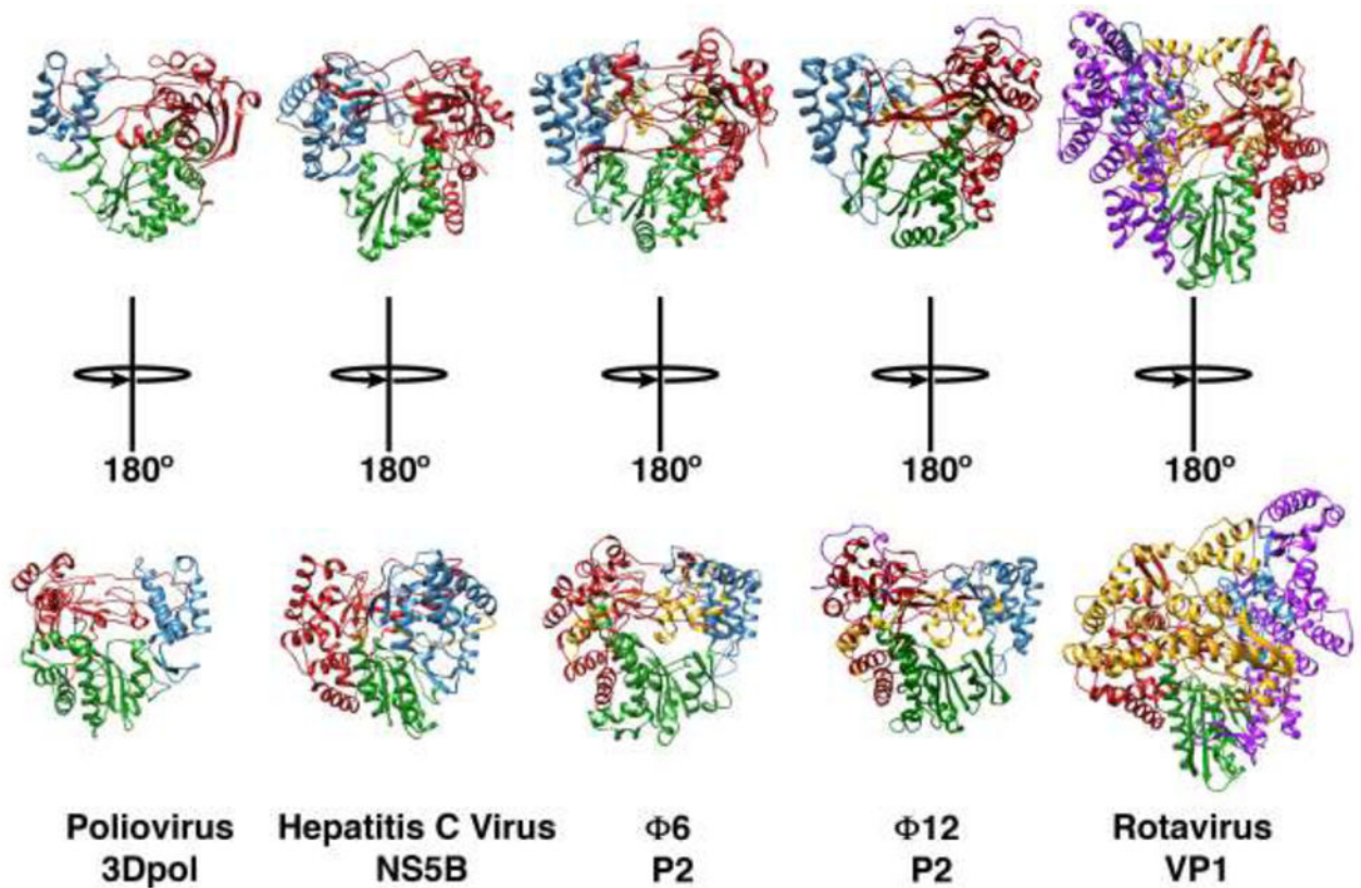
Figure 2. Structures of viral RNA-directed RNA polymerases
