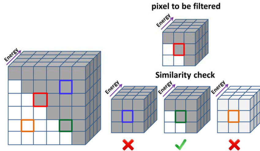
FIG. 2. MENLM also exploits spatial features to reduce noise and preserve edges. Different spatial features (e.g. 3x3 patches in the spatial domain) can be incorporated together with energy profiles in the similarity calculation, making the similarity evaluation robust to image noise. When filtering a pixel (red) on an edge, the spatial features helps to detect similar edge pixels (e.g., green) and exclude unlike ones (e.g. blue and orange).
