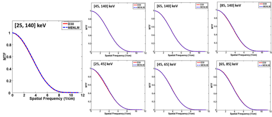
FIG. 6. Comparison of changes in in-plane spatial resolution between the FBP image (D30) and MENLM with 80% noise reduction for all threshold- and bin-based images.
