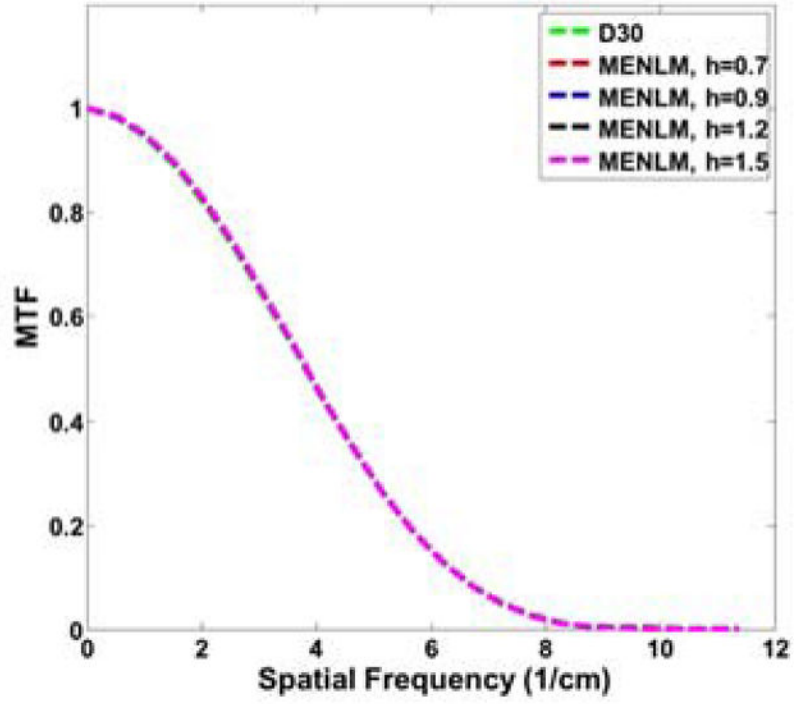
FIG. 5. Dependence of in-plane spatial resolution on filtering strength for Threshold 1 images [25,140 keV].
