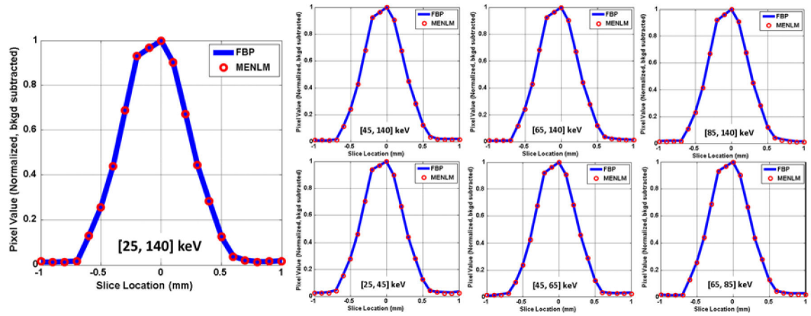
FIG. 7. Comparison of changes in cross-plane spatial resolution between the FBP image and MENLM with 80% noise reduction.
