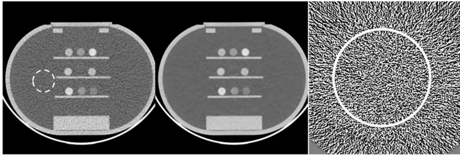
FIG. 8. Illustration of the calcium and iodine solution phantom used for the CT number accuracy evaluation. Left: Original FBP image of (85, 140) keV (W/L=400/40); Middle: MENLM image (W/L=400/40); Right: Difference image between FBP and MENLM images (W/L = 15/0 HU). The mean and standard deviation of CT numbers inside the dotted ROI were -0.3 \pm 19.2 and -0.4 \pm 4.1 HU for the FBP and MENLM images, respectively. No obvious structures were observed in the difference image. The mean and standard deviation of the CT number in the solid circle ROI was 0.2 \pm 15.8 HU, demonstrating no signal bias in the calcium and iodine solutions.
