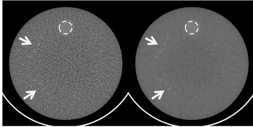
FIG. 10. Improved low-contrast resolution after MENLM filtering (right) comparing to the FBP image (left). Arrows indicate the locations of low-contrast objects (top: 6mm rods; Bottom: 5mm rods). The mean and standard deviation of CT numbers inside the dotted ROI were 99.3 \pm 5.5 (left) and 98.6 \pm 1.0 HU (right), respectively. W/L = 100/100 HU.
