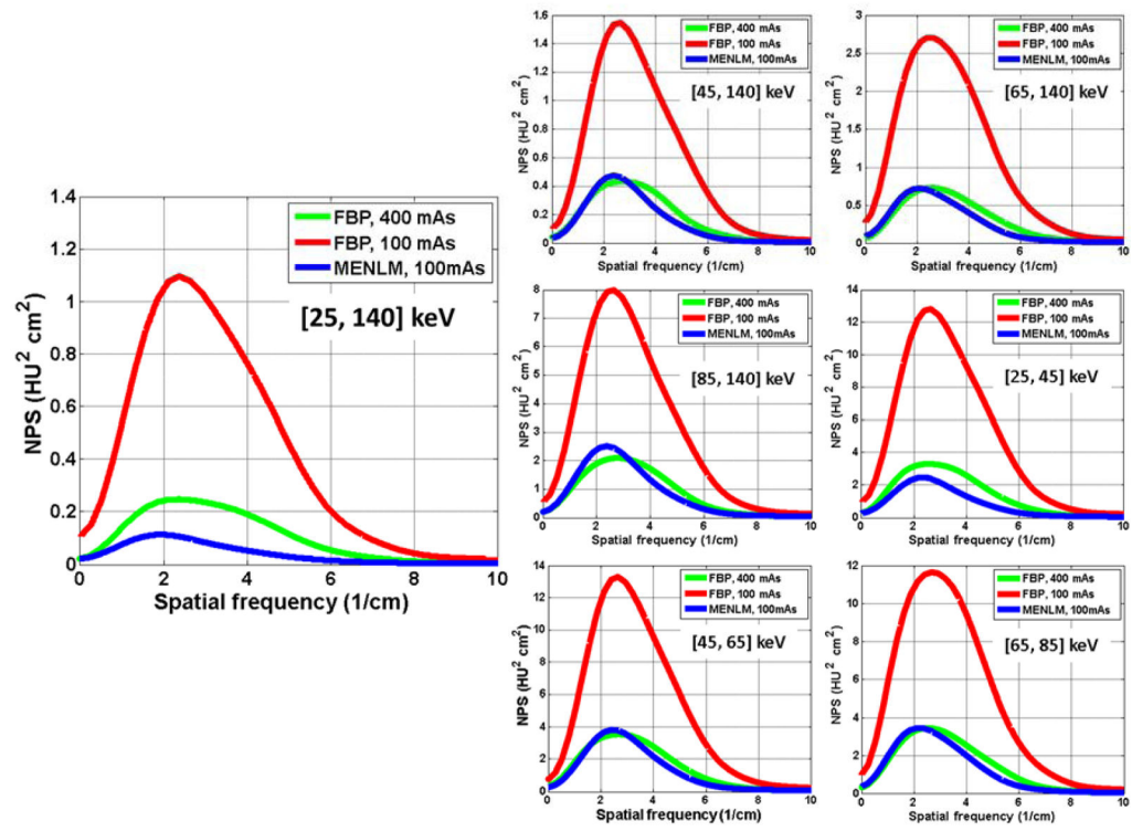
FIG. 3. Comparison of NPSs between the FBP images and MENLM filtered images with 50% noise reduction.
