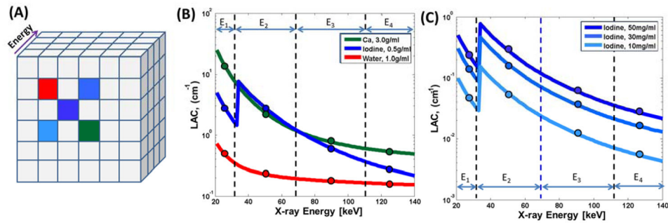
FIG. 1. MENLM exploits energy profiles to benefit similarity calculations between different pixels. (A). An illustration of MECT images, (B). Pixels with different material compositions and densities may have similar LACs in an energy channel (e.g. calcium and Iodine in E_2 and E_3 ). However, the different LAC values in other energy channels yield distinct energy profiles. (C). Pixels with the same material composition (blue blocks in sub-figure (A)) but different densities can still be differentiated because density differences also lead to different energy profiles in all energy channels.
