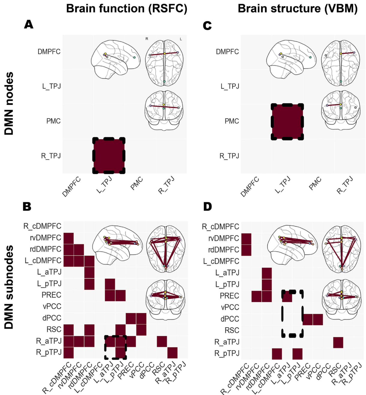
Figure 3. Studying node versus subnodes in the default mode network
