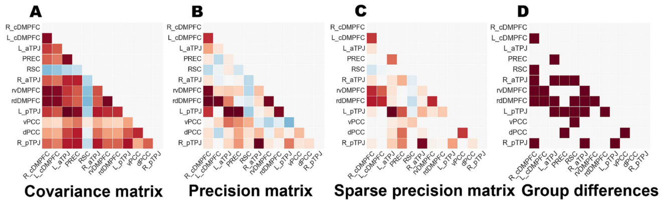
Figure 2. Network analysis workflow
