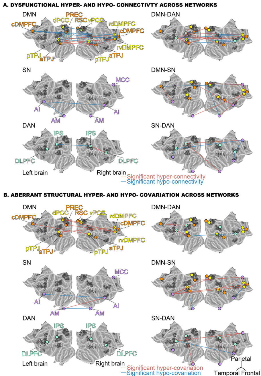
Figure 4. Dysfunctional connectivity and aberrant structural covariation across networks Depicts the significant increase ( red lines ) or decrease ( blue lines ) in functional connectivity (A) or in structural co-occurrence (B) comparing schizophrenic to healthy subjects in the across-network RSFC analyses (cf. SFig. 1). Circles represent regions of interest in the default mode network (DMN, orange ), the “DMN proper” ( yellow ), the saliency network (SN, purple ) and the dorsal attention network (DAN, light green ). The left column shows the differences within each network, while the right column displays differences between two networks. The connectivity findings show that the dysfunctional connectivities within the DMN include several subnodes that are not part of the “DMN proper”. While the functional
