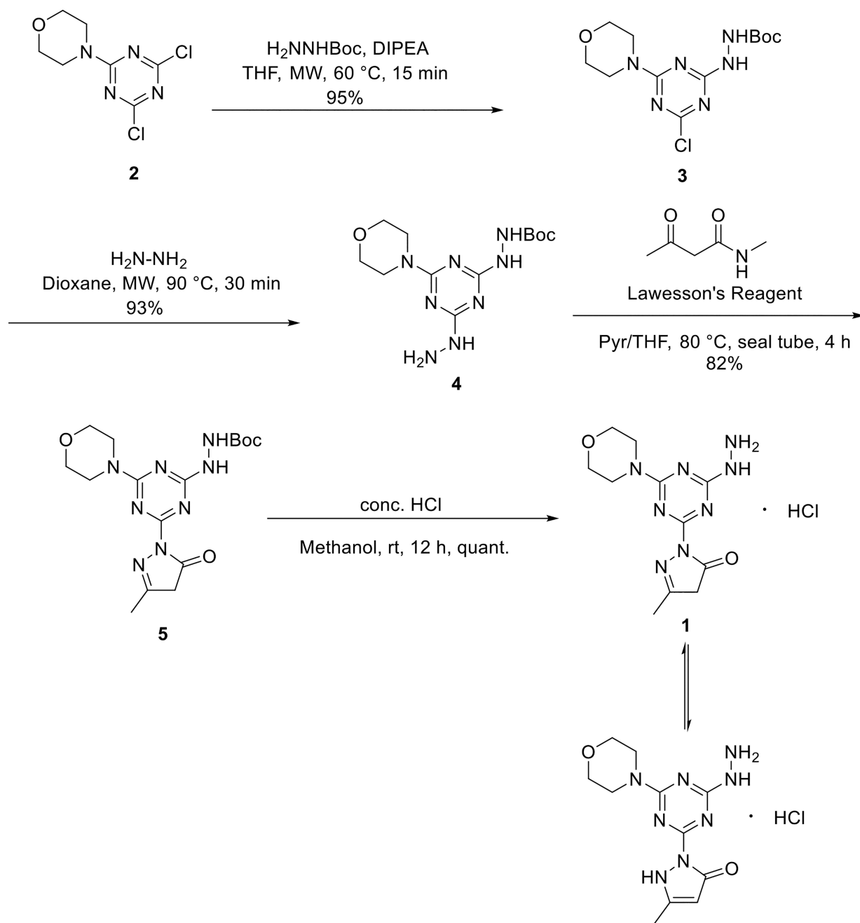
SCHEME 1. Synthesis of 1 .
