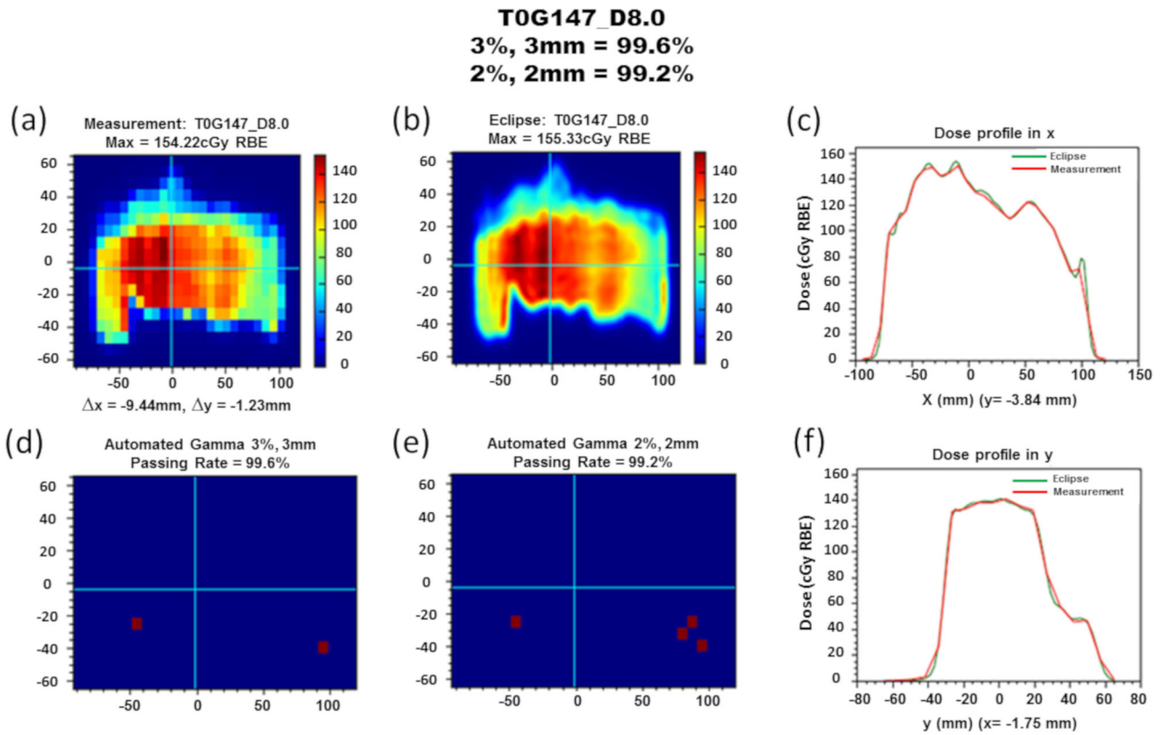
Figure 2: Automated gamma analysis summary for field T0G147 at a depth of 8.0 cm. (a) Planar dose measurement distribution with total lateral position correction of x = -9.44 mm and y = -1.23 mm. Prior to measurements, the detector was shifted ( x = 10.0 mm) to center the dose distribution, so x shifts by fitting algorithm are determined by delta of reported and detector-shifted values. (b) Planar dose distribution for the verification field at matching prescription depth. (c) Lateral dose profile along the x direction at y = -3.84 mm. (d) Automated \gamma -index analysis result with 3%, 3mm criteria indicating a 99.6% passing rate. (e) Automated \gamma -index analysis result with 2%, 2mm criteria indicating a 99.2% passing rate. (f) Lateral dose profile along the y direction at x = -1.75 mm.
