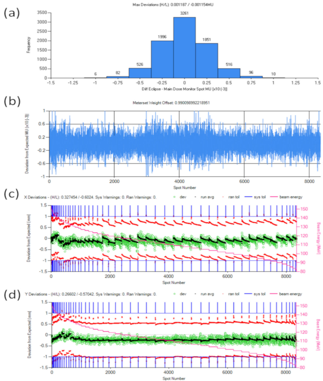
Figure A1: Log file analysis summary of a treatment field comparing the delivered spot MU and position to the planned version. (a) Histogram of spot MU deviations; (b) per spot MU deviation; (c) the per-spot position (green circles) and average (black dots) deviation in the horizontal aspect of the beams eye view, with systematic error tolerances represented by blue lines, random error tolerances represented by red points, and beam energy indicated by pink stair step and secondary vertical axis values; and (d) similar to (c) except showing the per spot position deviations in the vertical aspect of the beams eye view.
