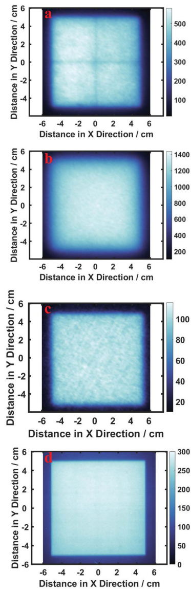
FIG. 9: Comparison between the 2D profiles of light field, Cherenkov, and dose of 10 \times 10 \text{ cm}^2 , 6MV, photon beam. (a): 2D profile of light field, (b): 2D profile of Cherenkov emission in an ABS board, (c): 2D profile of Cherenkov emission on a solid water phantom, (d): 2D profile of dose from GaF film measurement.
