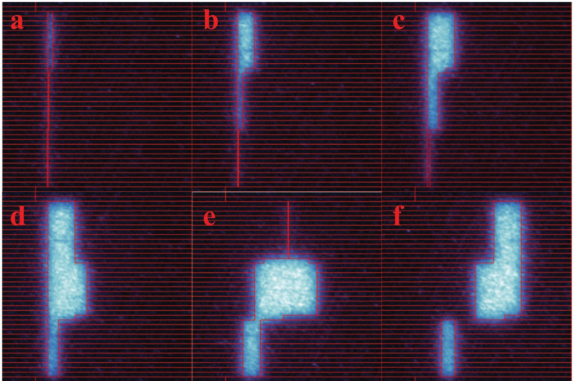
FIG. 7: Cherenkov images of IMRT QA plan on the isoplane, compared with MLC shapes projection, with leaves marked by red rectangles.
