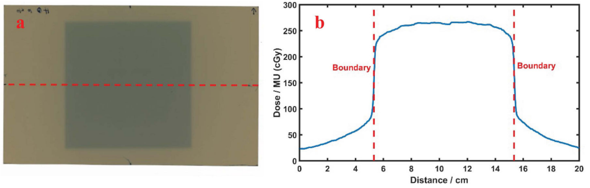
FIG. 4: Beam width measurement using GaF films (a): Film scan for 10cmx10cm beam and 5cmx5cm beam, with line profile region in 10cmx10cm beam (b): Dose profile along the line, with red lines representing the boundaries extracted through maximum derivative method.
